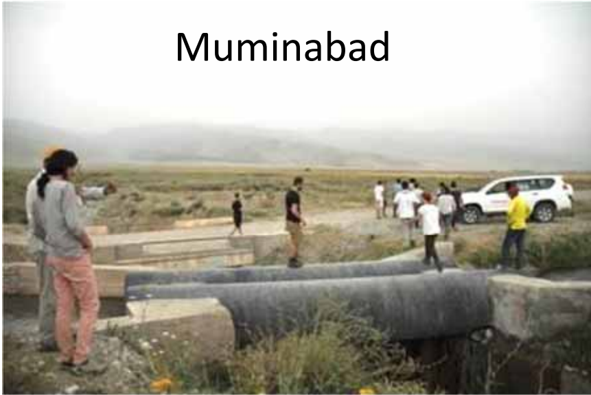
Reinforced outlet of a drainage canal built with the participation of local farmers
