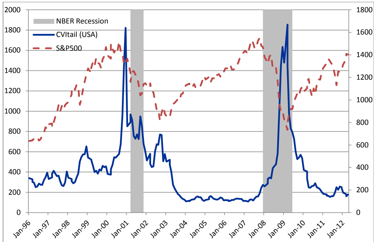
Figure 4: A comparison of CVI_{tail}(USA) and S&P 500 index during NBER recessions.
