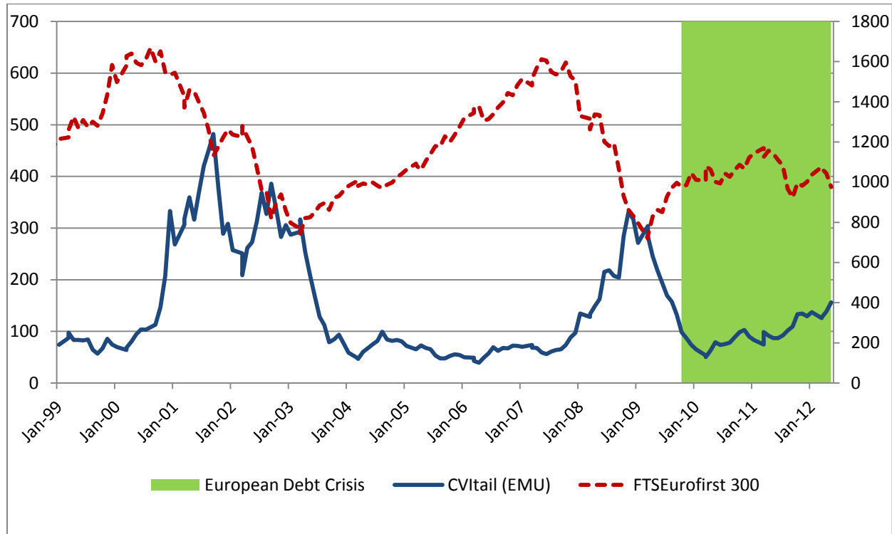
Figure 2: A comparison of the CVI_{tail}(EMU) and the FTSEurofirst300 during downturns.
