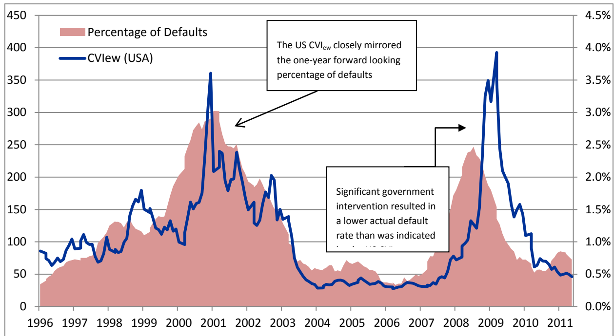
Figure 3: A comparison between CVI_{ew}(USA) and realized defaults in US.
