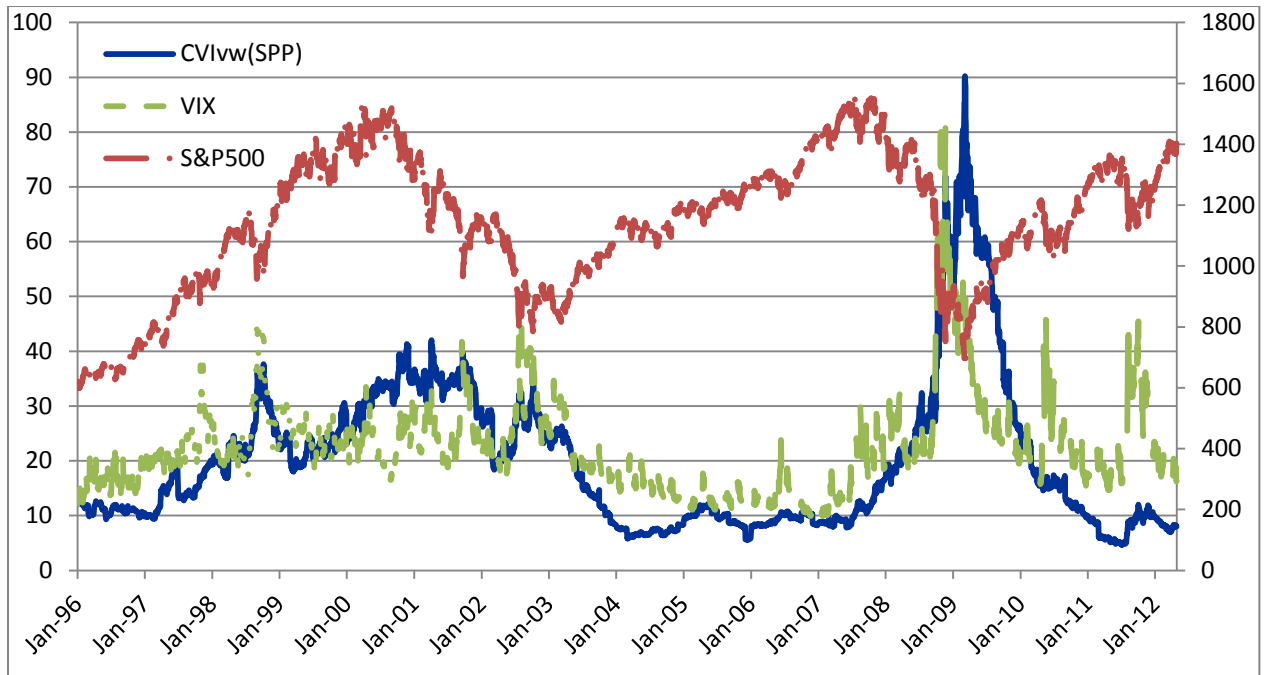
Figure 1: A comparison of the CVI_{vw} (SPP), VIX and S&P 500 index.
