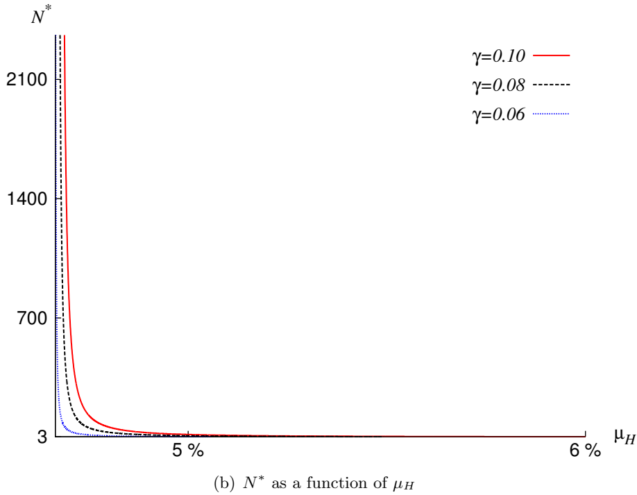
Fig. 2. A plot illustrating Proposition 5.4 where N^* is the minimal number of assets in the pool such that the equilibrium effort level is high. Parameter values: A_B = A_S = 0, r = 5\%, \gamma = 10\%, 8\%, 6\%, C = 2\% \frac{Nu}{r}, R/u = 50\%, u = 1, (a_L, \mu_L, \sigma_L) = (0.2, 0.04, 0.1), (a_H, \mu_H, \sigma_H) = (0.2, 0.04, 0.1) (except for the varying parameter).
