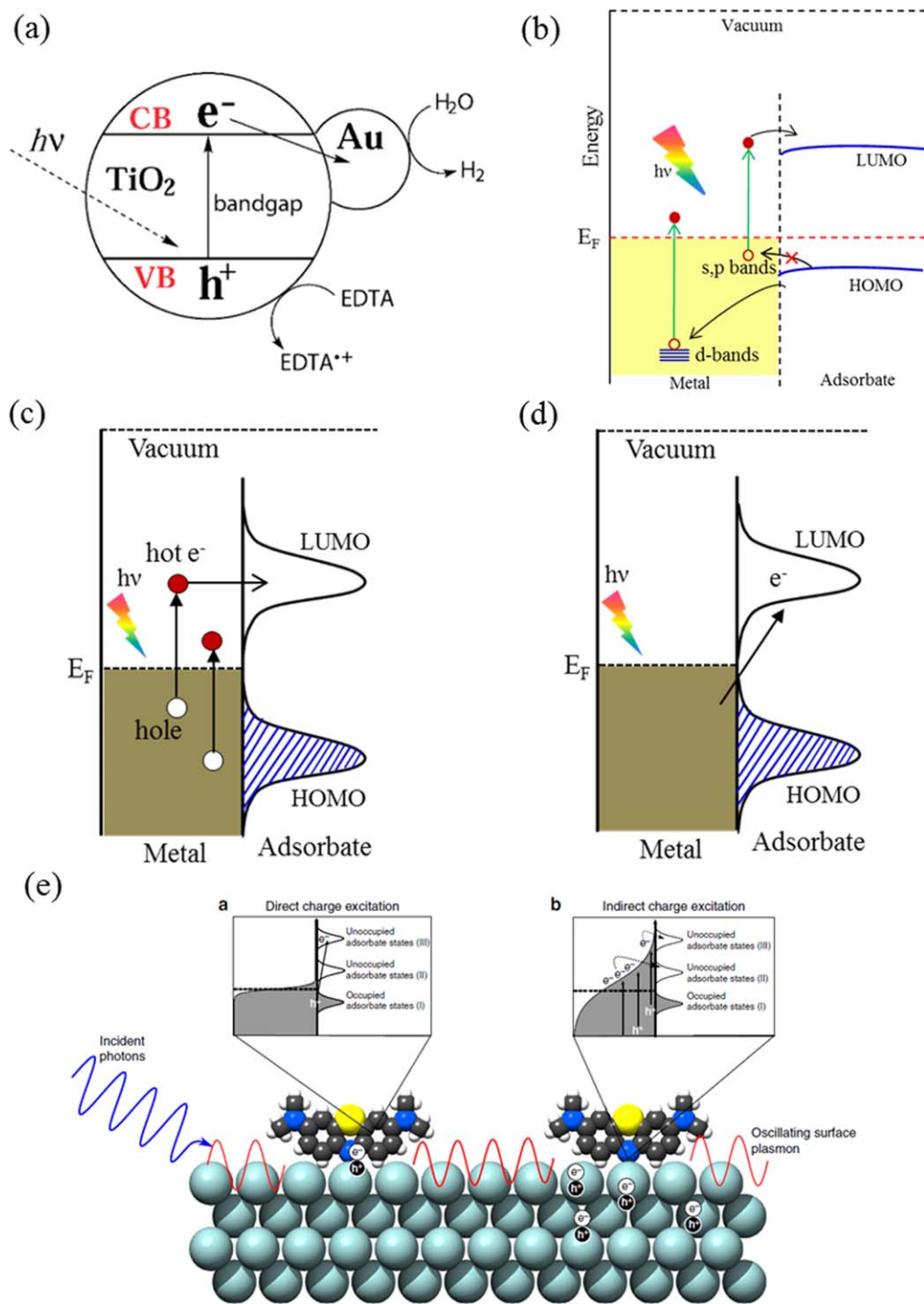
Figure 6. (a) Electron transfer from \text{TiO}_2 to Au under UV light excitation in the photocatalytic proton reduction reaction. Adapted with permission from Ref. 126. Copyright 2011 American Chemical Society. (b) Illustration of the electron transfer from HOMO of the adsorbate to the hot holes resulting oxidation reaction when their energy levels are matching. (c) Schematic of indirect charge-transfer mechanism. (d) Representation of direct charge-transfer mechanism. (e) Distinguishing direct and indirect charge transfer in Ag-MB system. Adapted with permission from Ref. 127. Copyright 2016 Nature Springer.
