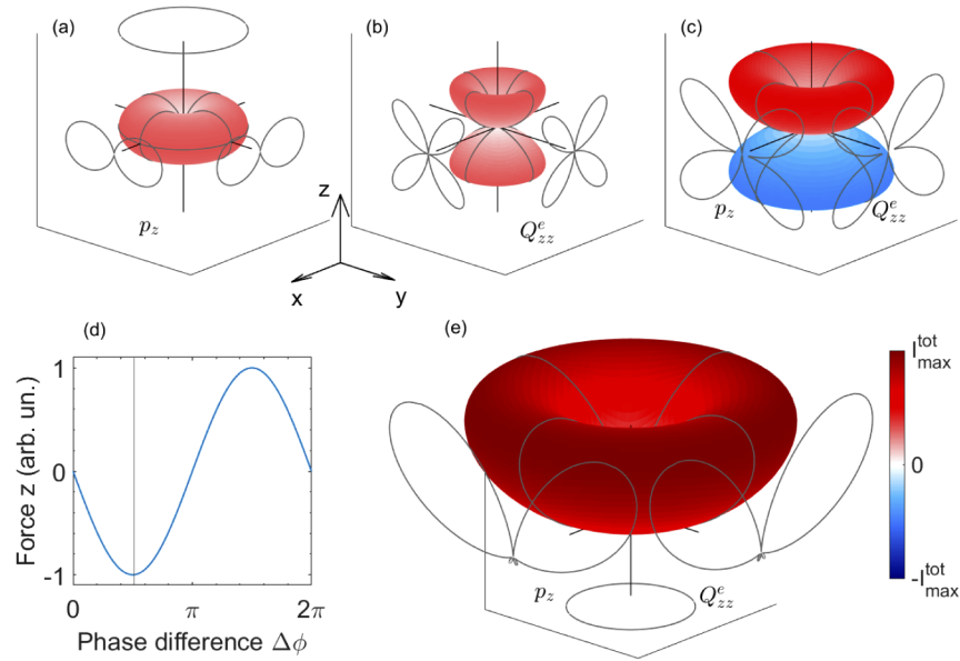
Fig. 3. Origin of the optical force resulting from the superposition of an electric dipole p_z with an electric quadrupole Q_{zz}^e , as a function of their relative phase difference \Delta\phi . (a) Radiation pattern for the electric dipole. (b) Radiation pattern for electric quadrupole. (c) Interference pattern for \Delta\phi = \pi/2 . (d) Normalized force dependency on the relative phase difference between both multipoles. (e) Total intensity distribution due to the sum of both multipoles. All patterns are normalized to the maximum intensity in panel (e). ( Visualization 4 ) Intensity distribution for different values of the relative phase difference.
