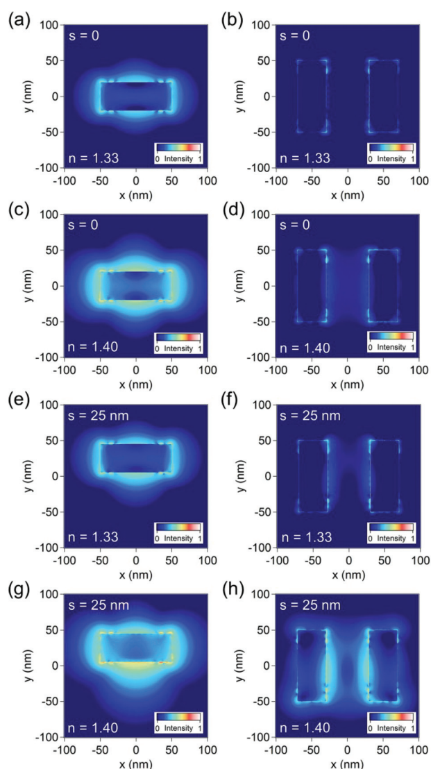
Fig. 4 SH near-field intensity maps (shown in a logarithmic scale) close to (a, c, e, g) the dipolar nanorod antenna and to (b, d, f, h) the two parallel nanorods evaluated for an incident wavelength \lambda = 860 nm for different cases: (a–d) s = 0 and (e–h) s = 25 nm. (a, b, e, f) n = 1.33 and (c, d, g, h) n = 1.40 . The same colorscale is used for the 8 maps.
