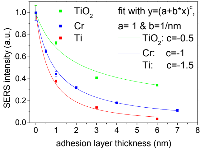
Figure S3. SERS intensity for Titanium, Titanium oxide and Chromium as adhesion material. The experimental data are fitted with the power law dependence (1+x/nm)^{-a} , where x is the layer thickness in nm and a the exponent describing the damping. a was fitted with 0.5 for TiO 2 , 1 for Cr and 1.5 for Ti. The normalized intensities correspond to the 1008 cm -1 Raman peak of a self-assembled benzene-ethane-thiol monolayer. Error bars represent the standard deviation of 16 spatially separated SERS measurements. The gold thickness for the periodic pattern was 50 nm and the gap size was 40 nm.
