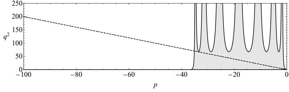
(a) Standard S-ROCK method ( s = 7 , \eta = 3.98 ).
