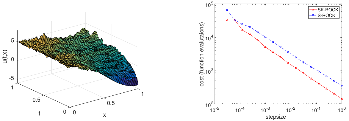
(a) One realization with SK-ROCK using \Delta t = 1/50 , \Delta x = 1/100 , s = 22 .
