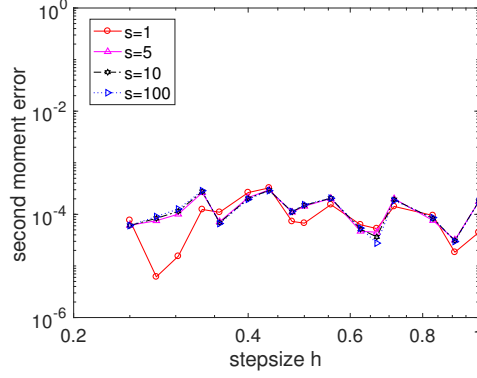
Figure 7: PSK-ROCK without damping ( \eta = 0 ). Second moment error of problem (54), with T = 10 , h = T/[2^{i/2}] , and s = 1, 5, 10, 100 , using M = 10^8 samples (the Monte-Carlo error has size M^{-1/2} = 10^{-4} ).
