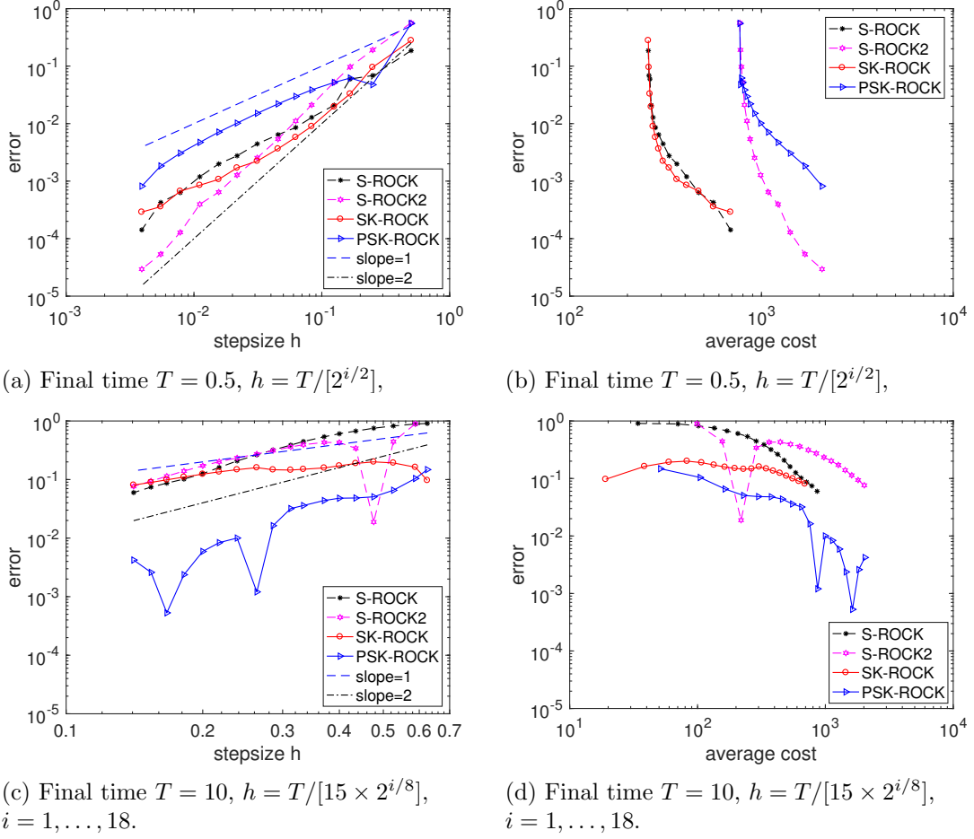
Figure 8: Second moment errors versus the average number of drift function evaluations for problem (55) using S-ROCK, S-ROCK2 and the new method SK-ROCK and its postprocessed version PSK-ROCK. We use discrete random increments and 10^8 samples.
