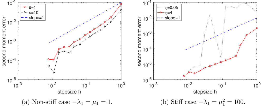
Figure 5: Nonlinear problem (52) with \nu = 2, \mu_2 = 0.5, \lambda_2 = -1 . Weak convergence plots using SK-ROCK for \mathbb{E}(X(T)^2) where T = 1, h = T/[2^{i/2}], i = 1, \dots, 14 , and 10^6 samples. For the stiff case (b), the method uses the following number of stages respectively: s = 8, 6, 5, 4, 4, 3, 3, 3, 2, 2, 2, 1, 1, 1 (with damping \eta = 0.05 ) and s = 13, 9, 8, 7, 6, 5, 4, 4, 3, 3, 3, 3, 2, 2 (with damping \eta = 4 ).
