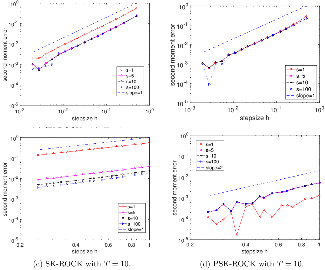
Figure 6: Linear additive problem (54). Second moment error \mathbb{E}(X(T)^2) for for short time T = 0.5 (top pictures) and long time T = 10 (bottom pictures) without (SK-ROCK) or with a postprocessor (PSK-ROCK). where, h = T/[10 \times 2^{i/8}] for T = 10 , and h = T/[2^{i/2}] for T = 0.5 with i = 1, \dots, 16 , and 10^8 samples.
