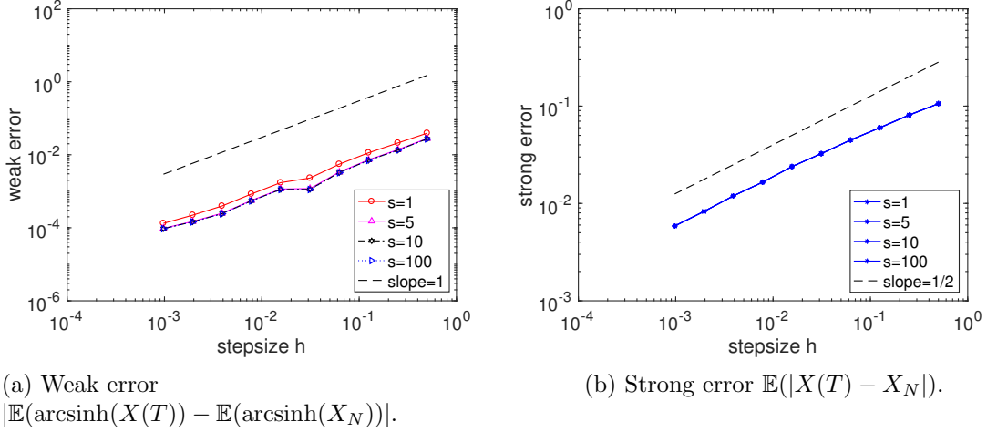
Figure 4: Nonlinear problem (51). Strong and weak convergence plots using SK-ROCK with final time T = 1 , stepsizes h = 2^{-p} , p = 1..10 , 10^4 samples and number of stages s = 1, 5, 10, 100 .
