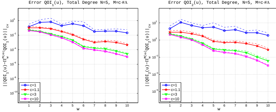
FIGURE 3.9. Example 3: the Darcy model. \beta = 5 .
