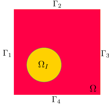
FIGURE 3.1. Square domain \Omega with a circular inclusion \Omega_I .
