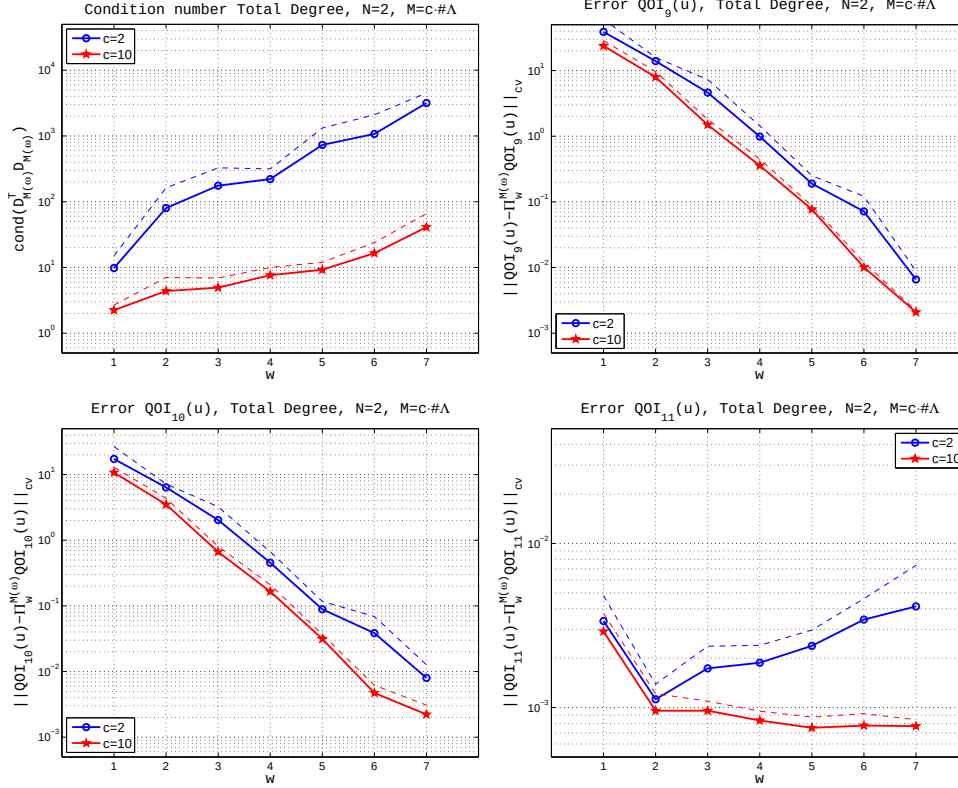
FIGURE 3.13. Example 5. Condition number and approximation errors averaged over 5 repetitions, M = c \cdot \#\Lambda .
