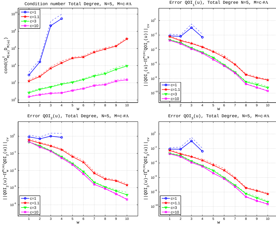
FIGURE 3.8. Example 3: the Darcy model. \beta = 2 .
