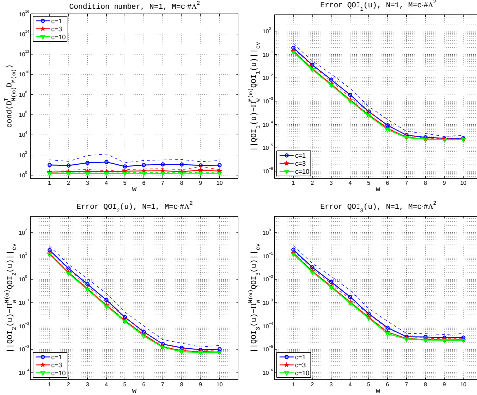
FIGURE 3.5. Example 2. Condition number and approximation errors averaged over 100 repetitions, M = c \cdot (\#\Lambda)^2 .
