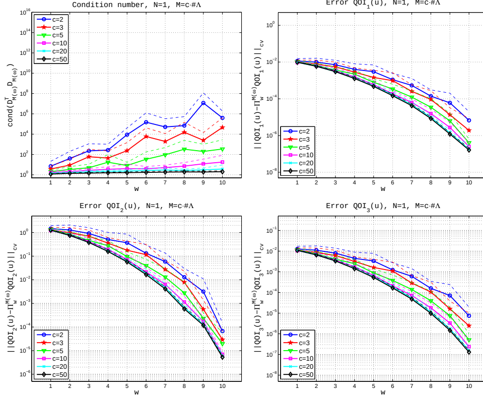
FIGURE 3.2. Example 1. Condition number and approximation errors averaged over 100 repetitions, M = c \# \Lambda .
