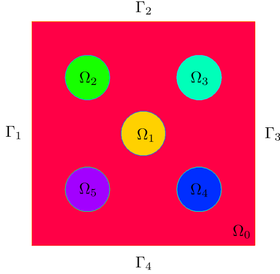
FIGURE 3.7. Domain with 5 inclusions \Omega_1, \Omega_2, \Omega_3, \Omega_4, \Omega_5 with random diffusivity for problem (3.2).
