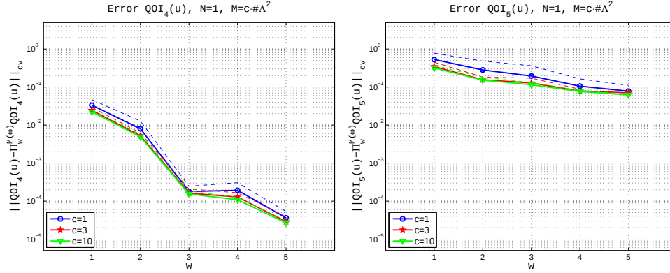
FIGURE 3.6. Example 2. Approximation errors averaged over 100 repetitions, M = c \cdot (\#\Lambda)^2 .
