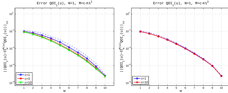
FIGURE 3.3. Example 1. Approximation errors averaged over 100 repetitions, M = c \cdot (\# \Lambda)^2 (left), M = c \cdot (\# \Lambda)^3 (right).
