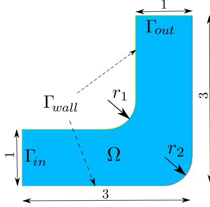
FIGURE 3.12. Geometry of the domain \Omega in Example 5.
