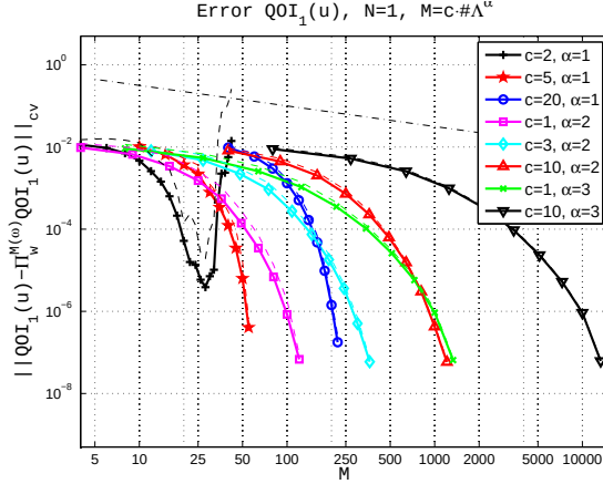
FIGURE 3.4. Example 1. Approximation errors vs M for different choices of the sample size, M = c \cdot (\#\Lambda)^\alpha . Same data as in Fig. 3.2 (top-right) and Fig. 3.3.
