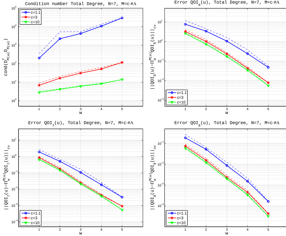
FIGURE 3.11. Example 4. Condition number and approximation errors averaged over 100 repetitions, M = c \cdot \#\Lambda .
