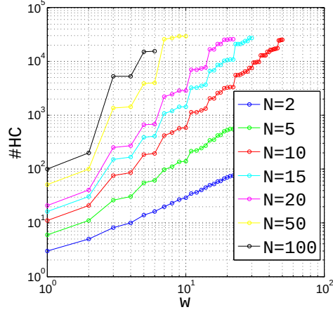
FIGURE 2.1. Dimension of the HC space, N = 2, 5, 10, 15, 20, 50, 100 .
