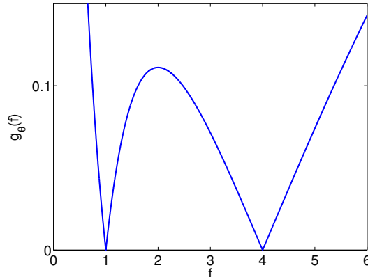
FIG. 4.1. Function g_\theta(f) from the proof of Corollary 4.3 for \theta = 4 .
