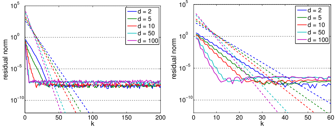
FIG. 5.3. Norm of residuals for rational Krylov subspace method with shifts \infty and \sigma_{opt} . Solid lines correspond to computed residuals and dashed lines correspond to the bound obtained from Corollary 4.3. Left: Discrete Laplace. Right: Diagonal matrix. (5.2).
