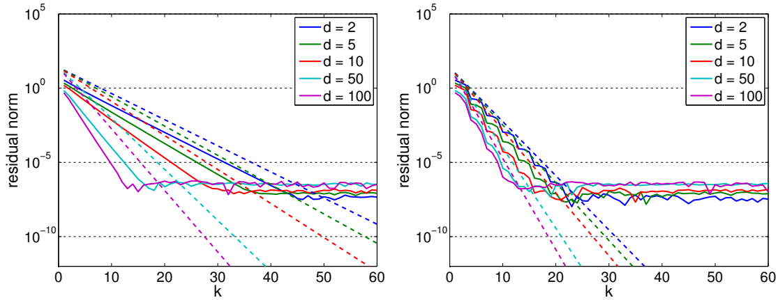
FIG. 5.4. Norm of residuals for rational Krylov subspace method with optimal ADI shifts. Solid lines correspond to computed residuals and dashed lines correspond to the bound from Theorem 3.2. Left: One shift. Right: Three shifts.
