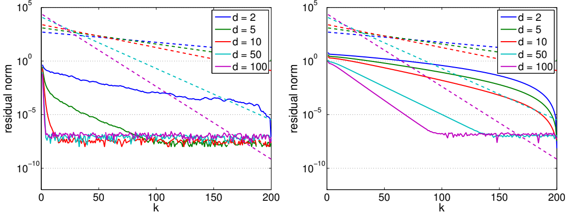
FIG. 5.1. Norm of residuals for standard Krylov subspace method. Solid lines correspond to computed residuals and dashed lines correspond to the bound obtained from Corollary 4.1. Left: Randomly chosen right-hand side. Right: Particularly constructed right-hand side (5.1).
