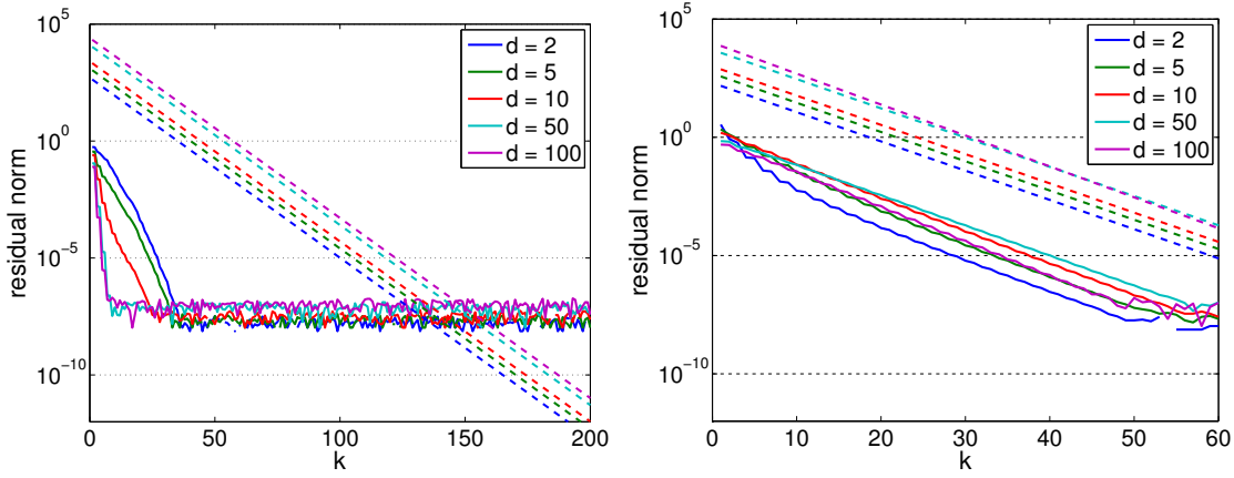
FIG. 5.2. Norm of residuals for extended Krylov subspace method. Solid lines correspond to computed residuals and dashed lines correspond to the bound obtained from Corollary 4.2. Left: Discrete Laplace. Right: Diagonal matrix (5.2).
