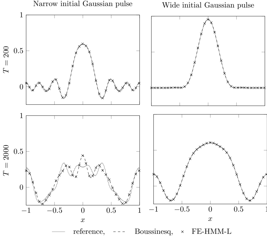
FIG. 5.7. One-dimensional periodic medium. The solutions u^\varepsilon , u^{\text{eff}} , and u_H are shown for two different initial conditions at T = 200 (top) and T = 2000 (bottom). Left: narrow initial Gaussian pulse ( \sigma^2 = 1/100 ); right: wide initial Gaussian pulse ( \sigma^2 = 1/20 ). In the lower left frame u^{\text{eff}} and u_H coincide, yet both differ from u^\varepsilon .
