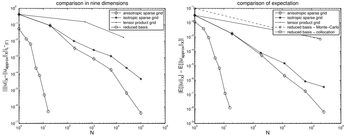
Figure 7.5: Comparison for convergence rate of the error |||u||_X - ||u_{approx}||_X||_{L^\infty(\Gamma)} (left) and the expectation |\mathbb{E}[||u||_X] - \mathbb{E}[||u_{approx}||_X]| (right) between the true and the approximate solutions in 9D
