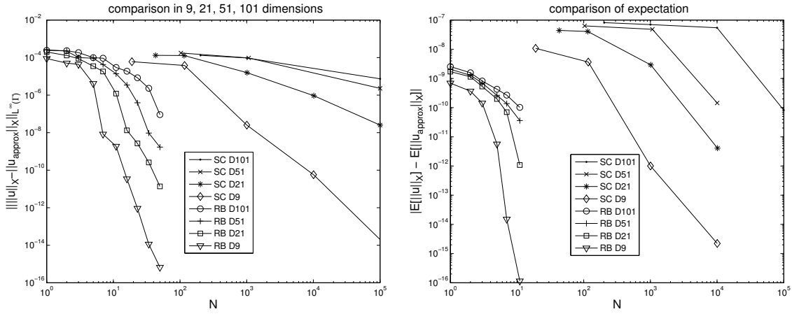
Figure 7.6: Comparison for convergence rate of \| |u|_X - |u_{approx}|_X \|_{L^\infty(\Gamma)} (left) and the expectation |E[|u|_X] - E[|u_{approx}|_X]| (right) between the anisotropic sparse grid stochastic collocation (SC) approximation and the reduced basis (RB) approximation in high dimensions 9D, 21D, 51D and 101D
