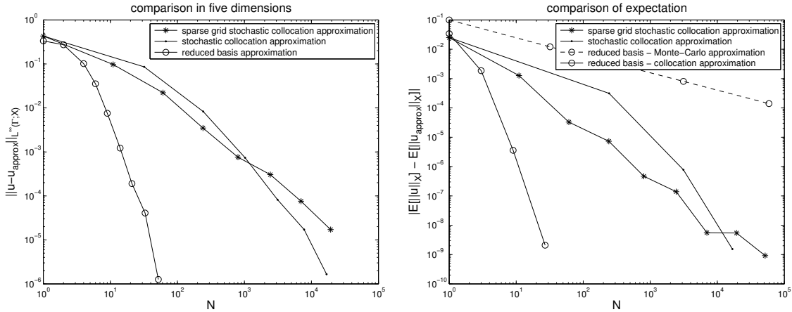
Figure 7.3: Comparison for convergence rate of the error \|u - u_{approx}\|_{L^\infty(\Gamma; X)} (left) and the expectation |\mathbb{E}[\|u\|_X] - \mathbb{E}[\|u_{approx}\|_X]| (right) between the true and the approximate solution in 5D
