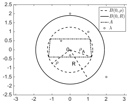
Figure 2: Five poles of a meromorphic mapping \mathcal{T} are represented (small circles). The disk \mathcal{B}(0, R) (solid line) contains exactly three poles of \mathcal{T} . We consider a Padé approximant \mathcal{T}_{[M/N]} with N = 3 . We are interested in approximating the map \mathcal{T} inside the compact subset A . Hence, we take \rho = \rho_A + \varepsilon , with 0 < \varepsilon \ll 1 , and we construct the disk \mathcal{B}(0, \rho) (dashed line). The rate of approximation of the Padé approximant is (\frac{\rho}{R})^{M+1} ; see Theorem 5.1.
