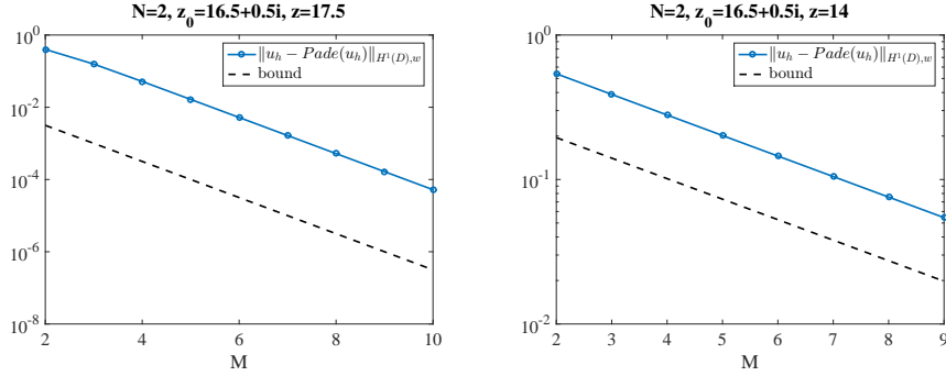
Figure 6: Comparison between the computed error \|u_h(z, \cdot) - u_{P,h}(z, \cdot)\|_{V, \sqrt{\operatorname{Re}(z_0)}} (solid line) and the predicted slope of convergence \left(\frac{\rho}{R}\right)^{M+1} (dashed line) proved in Corollary 6.1. Here K = [14, 19] , and z_0 = 16.5 + 0.5i . Moreover, \rho = |16.5 + 0.5i - 17.5| ( \rho = |16.5 + 0.5i - 14| , respectively) and R = |16.5 + 0.5i - 20| = |16.5 + 0.5i - 13| in the left (right, respectively) picture.
