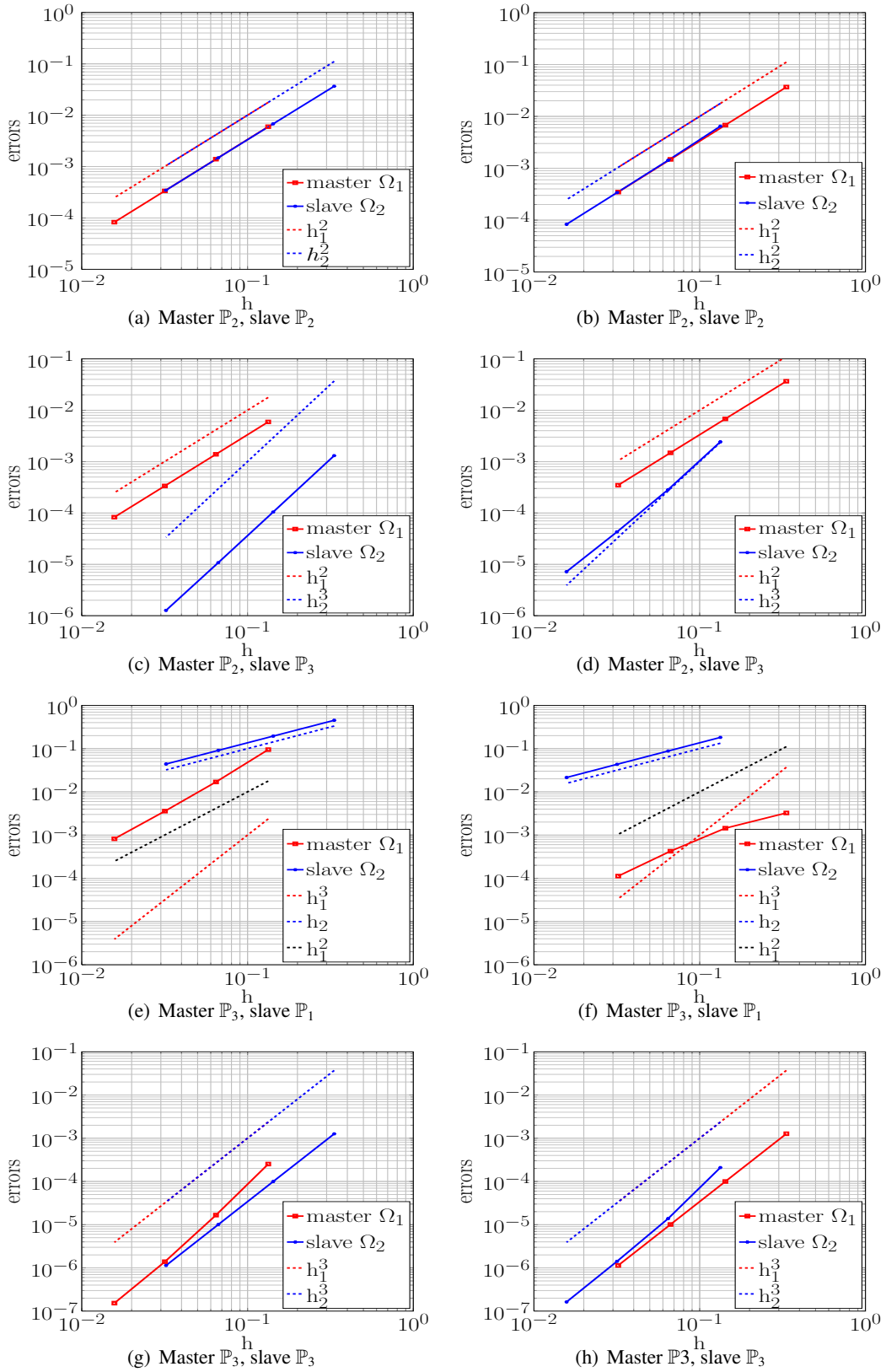
Figure 5: FEM-FEM coupling: orders of convergence obtained using Lagrangian interpolants and non-conforming meshes with aspect ratio 2. Left column using Set C, right column using Set D (see Table 2).
