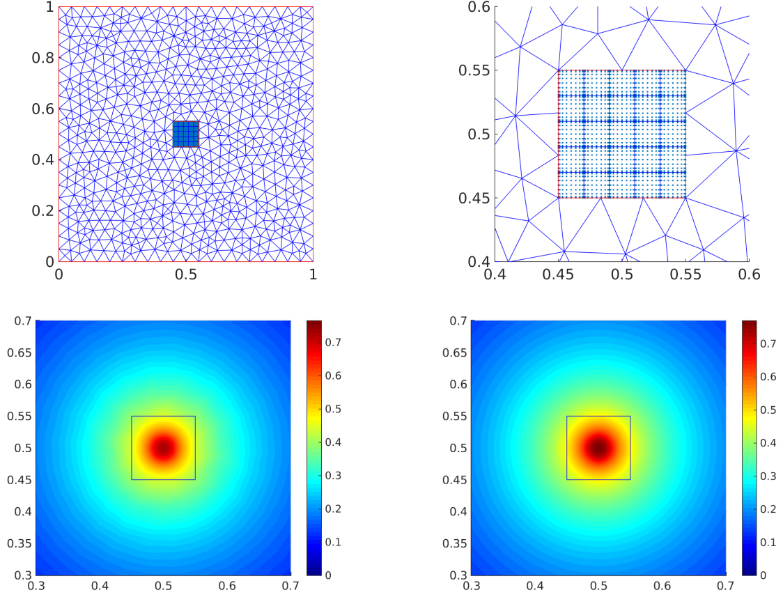
Figure 14: At top, the mesh used in the simulation of the diffusion of pollutant concentration (the right picture is a zoom of the left one). At bottom, the numerical solution obtained by both the INTERNODES with Lagrange interpolant as intergrid operator (at left) and by monodomain conforming SEM \mathbb{Q}_{32} on the whole \Omega (at right).
