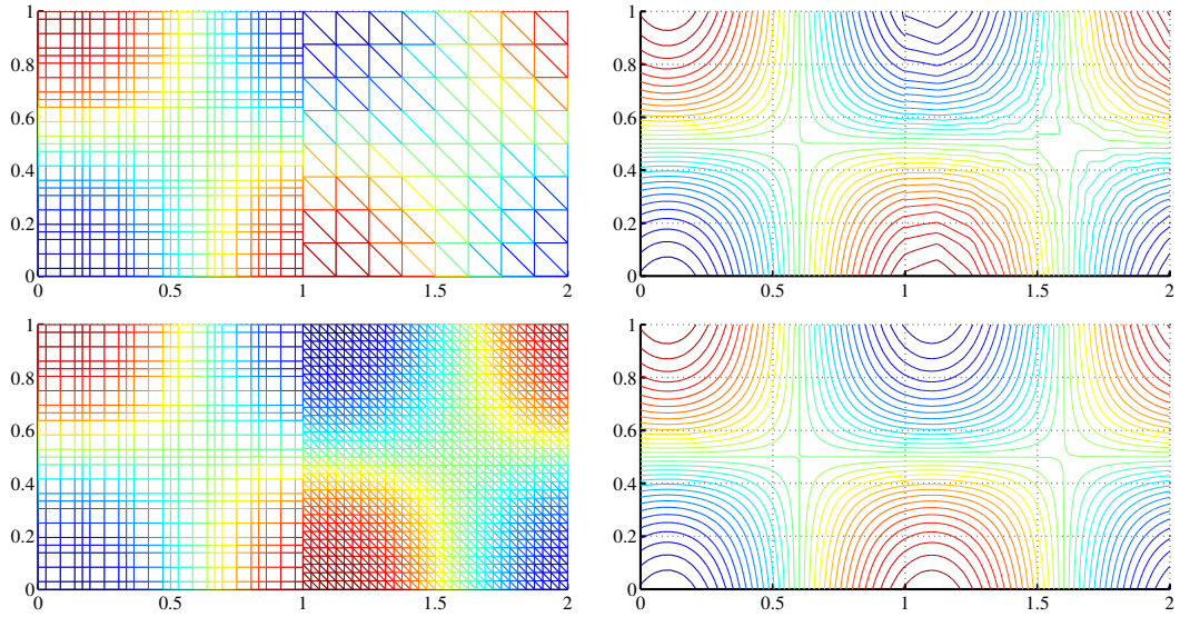
Figure 10: SEM-FEM coupling. Meshes (at left) and solution contours (at right) obtained using \mathbb{Q}_4 in \Omega_1 (master) and \mathbb{P}_1 in \Omega_2 (slave). At top h_2 = 1/8 , at bottom h_2 = 1/32 .
