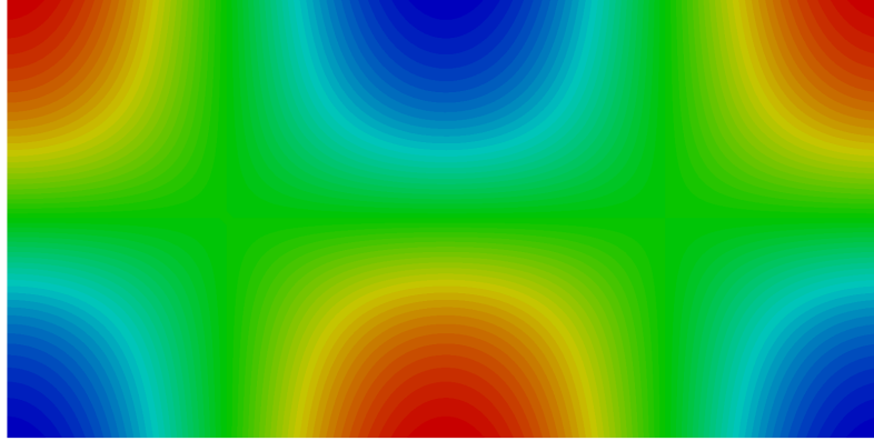
Figure 4: Solution u(x, y) = \arctan(4(y - 0.5)) \cos(\pi x) of problem (42).
