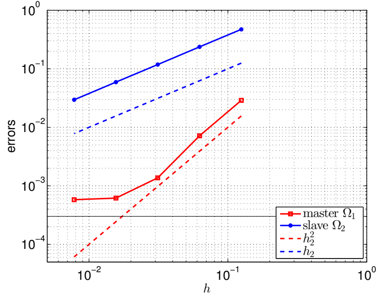
Figure 9: SEM-FEM coupling. H^1 norm errors vs. h_2 when \mathbb{Q}_4 are used in \Omega_1 (master) with fix h_1 = 1/6 , and \mathbb{P}_1 are used in \Omega_2 (slave). The black line denotes the error obtained by discretizing the global domain by conforming \mathbb{Q}_4 SEM.
