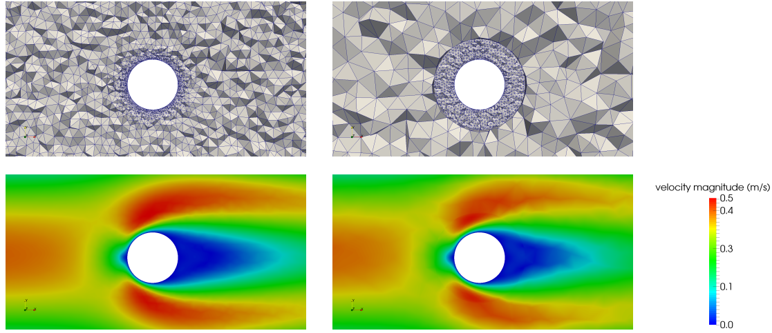
Figure 17: Zoom of the meshes and the velocity fields in the region close to the cylinder on a cut plane at z = 0.205\text{ m} : in the first row we show the meshes used for the numerical simulations. In the second row we plot the velocity fields obtained.
