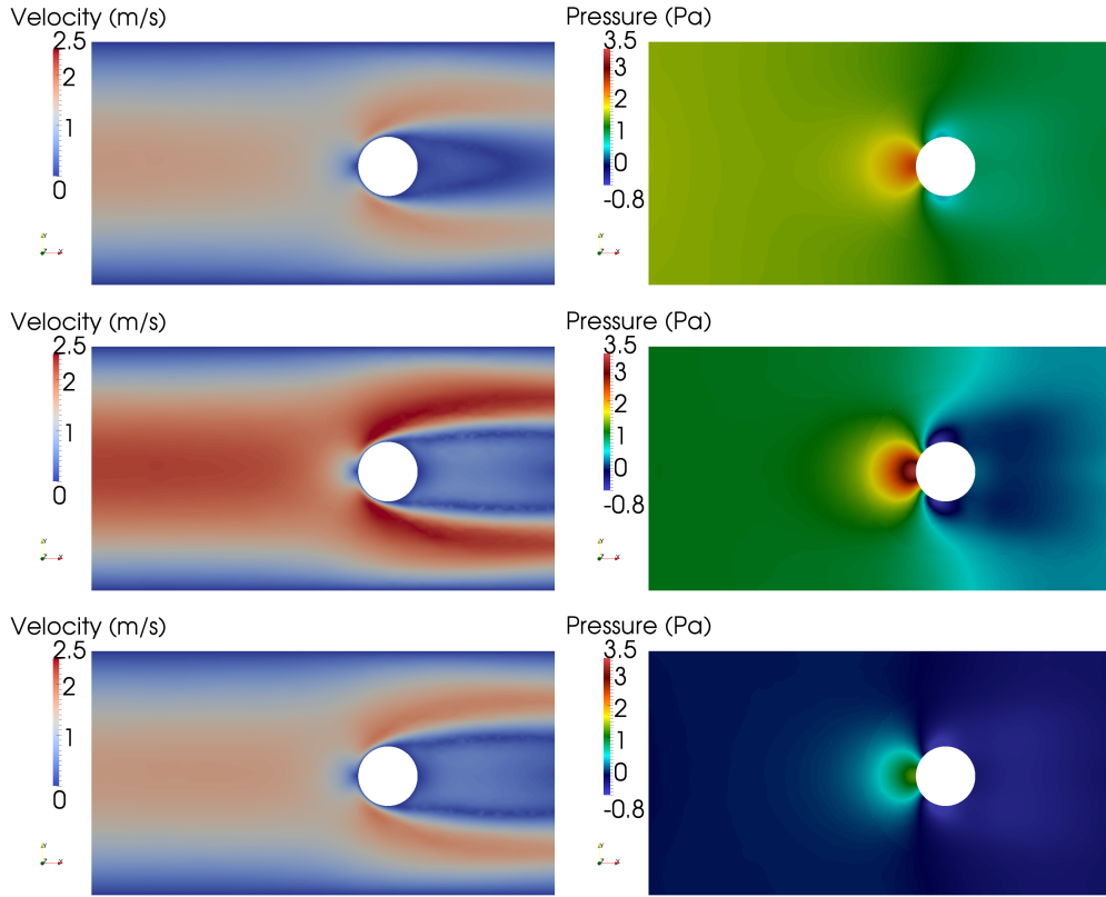
Figure 19: Visualization of the numerical solution obtained at times t = 2 s (top row), t = 4 s (middle row) and t = 6 s (bottom row). On the left column we report the fluid velocity while on the right the fluid pressure.
