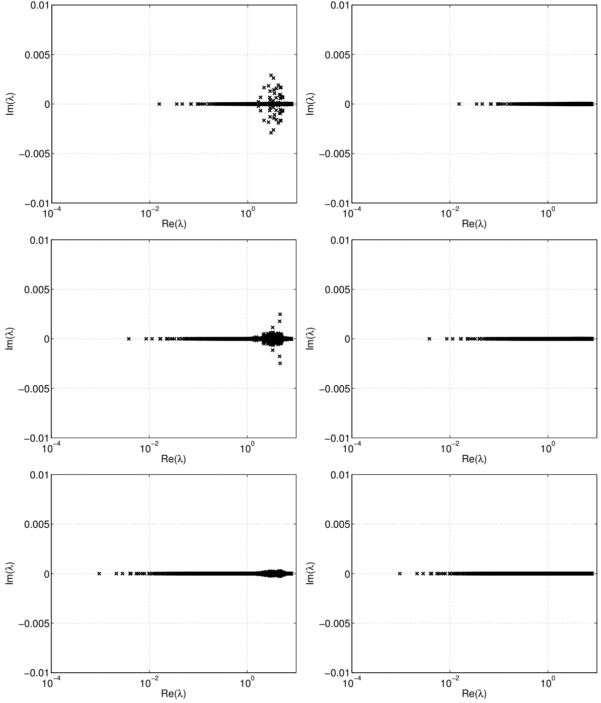
Figure 3: The spectra of the Dirichlet stiffness matrix of system (29) for INTERNODES (left) and mortar (right), corresponding to three different structured triangulations (Set D of Table 2, k = 16 (top), 32 (middle), 64 (bottom)).
