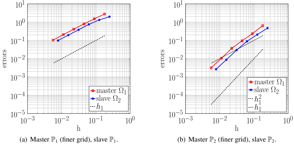
Figure 13: Rates of convergence in H^1 norm using geometrically non-conforming interfaces.
