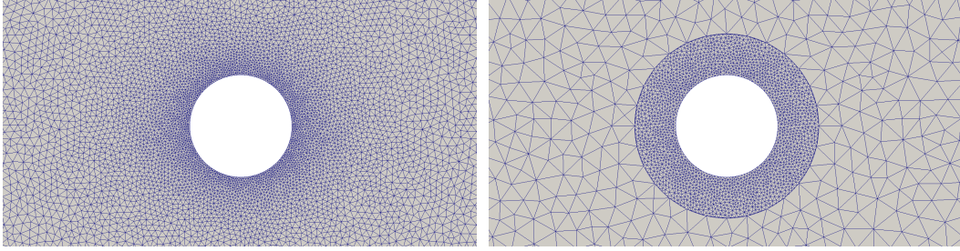
(a) Boundary layer refinement obtained by progressive (b) Independent meshes for the far field and the reduction of the mesh size (cross section). boundary layer zones (cross section).
