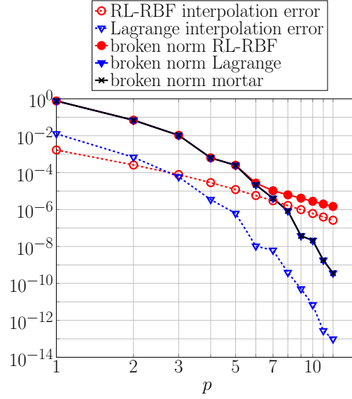
Figure 8: Comparison between PDE approximation errors and interpolation errors for SEM-SEM couplings 8 \times 8 and 6 \times 6 spectral elements are used in the master and in the slave subdomains, respectively.
