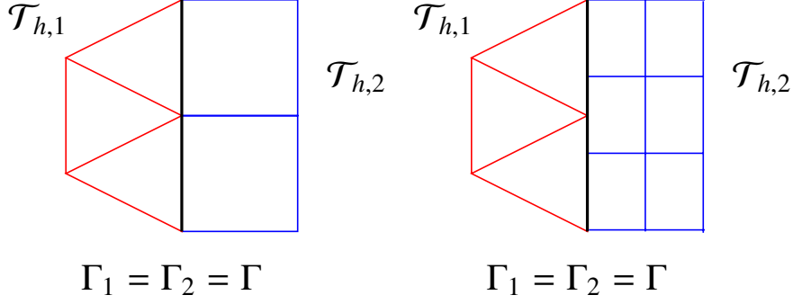
Figure 1: Conforming (at left) and non-conforming (at right) grids at the interface when d = 2 .
