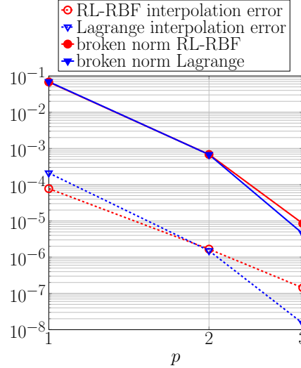
Figure 6: Comparison between PDE approximation errors and interpolation errors for \mathbb{P}_p - \mathbb{P}_p FEM, and non-conforming meshes (set D of Table 2 and k = 64 ).
