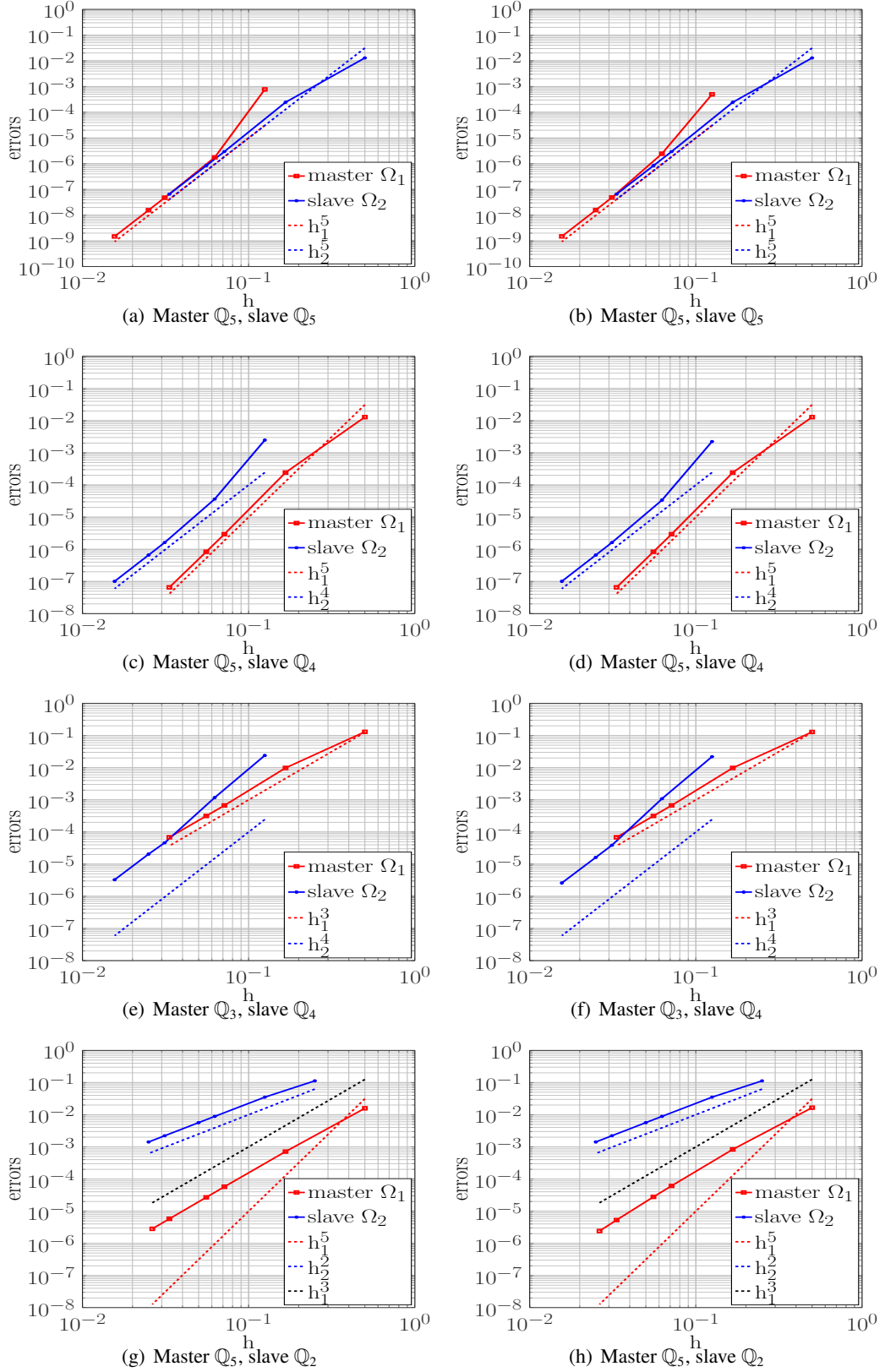
Figure 7: Convergence history with respect to the mesh sizes h_1 and h_2 for INTERNODES (left) and mortar (right) approaches. SEM discretization. First line: Set C; second line: Set D; third line: Set D; fourth line: Set A.
