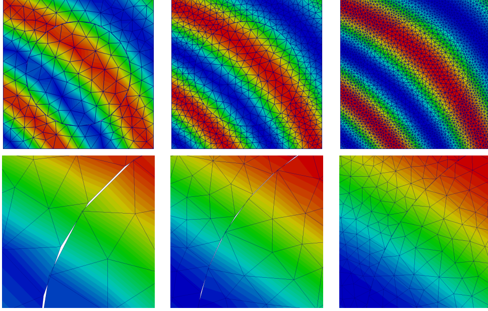
Figure 12: Solutions obtained using \mathbb{P}_1 - \mathbb{P}_1 finite elements for the master and slave domains using meshes of increasing refinement that are geometrically non-conforming. In the top row we show the numerical results on the whole domain while in the bottom row a zoom of the solution close to the interface is displayed.
