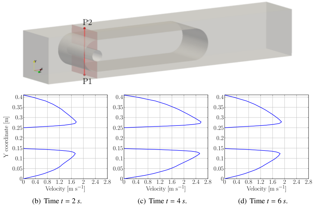
Figure 20: Plot over line, between points P1 = (0.5, 0, 0.205) and P2 = (0.5, 0.41, 0.205) , of the flow velocity at different times.
