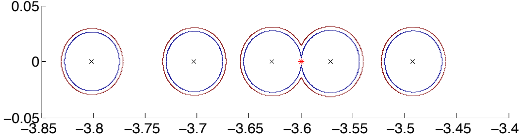
Figure 1: Contours of the pseudospectra for the nonlinear eigenvalue problem (30), with the eigenvalues marked by crosses. The inner contour corresponds to the \epsilon -pseudospectrum for \epsilon equal to the distance to a nearest nonlinear eigenvalue problem with a multiple eigenvalue. Two components coalesce as expected, and the point of coalescence marked with an asterisk is the multiple eigenvalue of a nearest nonlinear eigenvalue problem.
