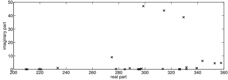
Figure 2: Eigenvalues of nonlinear eigenvalue problem (31).
