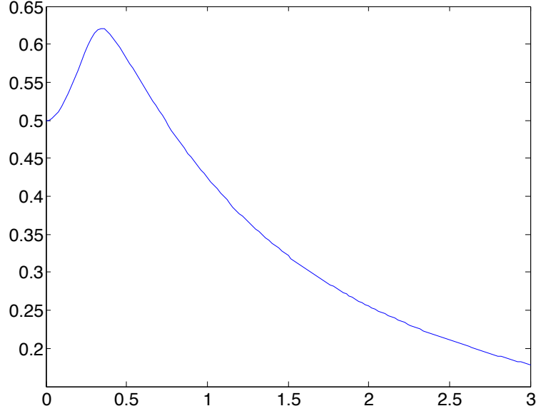
Figure 3: The plot of \sigma_{-2}(\mathcal{T}(\mu, \gamma, T)) with respect to \gamma \in [0, 3] for \mu = [\mu_1^{(2)}, \mu_2^{(2)}] where \mu_1^{(2)}, \mu_2^{(2)} are as in Table 1
