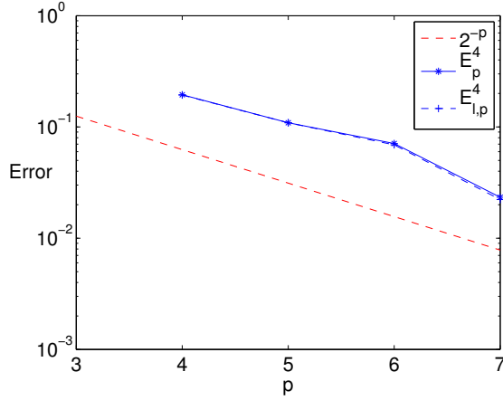
Figure 5: Numerical convergence for 4-mode truncation. On the horizontal axis we monitor the accuracy of the micro-timestep and on the vertical axis we measure the error as given by (64a) and (64b) with M = 4 .
