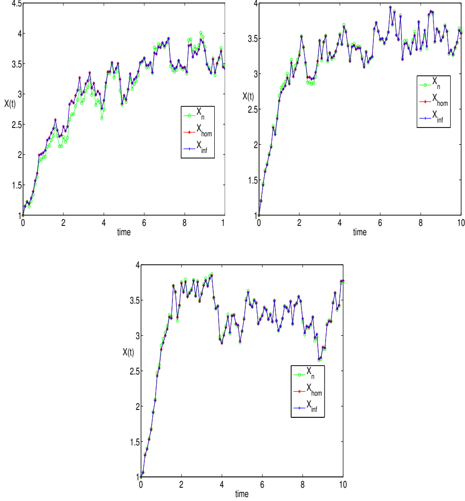
Figure 2: Euler-Maruyama methods (59) (solution denoted X_n ), (63) (solution denoted X_{n,\text{hom}} ) and (62) (solution denoted X_{n,\text{inf}} ) for three paths (upper panel, left p = 3 for X_n , upper panel right p = 4 for X_n , lower panel p = 5 for X_n ). We use 2-mode truncation for (59) and (63).
