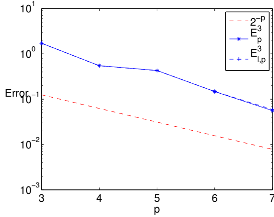
Figure 4: Numerical convergence for 3-mode truncation. On the horizontal axis we monitor the accuracy of the micro-timestep and on the vertical axis we measure the error as given by (64a) and (64b) with M = 3 .
