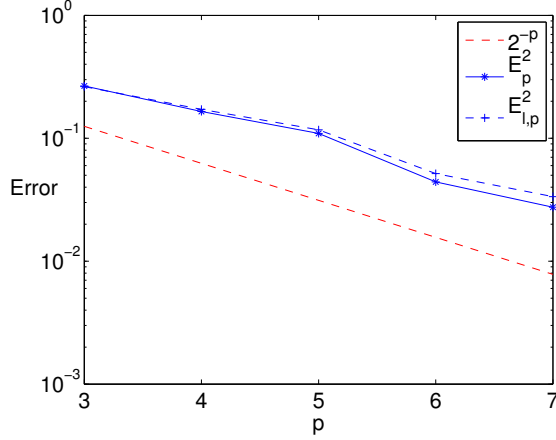
Figure 1: Numerical convergence for 2-mode truncation. On the horizontal axis we monitor the accuracy of the micro-timestep and on the vertical axis we measure the error as given by (64a) and (64b) with M = 2 .
