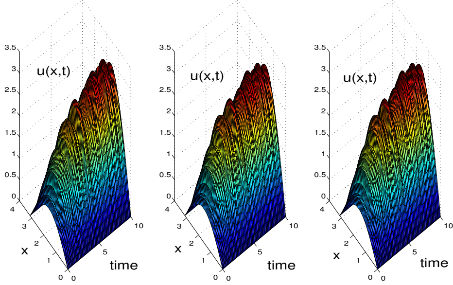
Figure 3: Approximation (57) of the solution u(x, t) of the SPDE; u(\cdot, t) \simeq X_n(t) \sin(\pi \cdot) (left figure p = 3 ), u(\cdot, t) \simeq X_{n,\text{hom}}(t) \sin(\pi \cdot) (middle figure) and u(\cdot, t) \simeq X_{n,\text{inf}}(t) \sin(\pi \cdot) (right figure).
