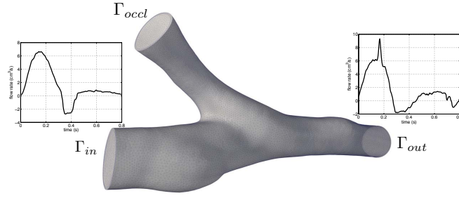
Figure 7: Femoropopliteal bypass geometry. Graph of the inlet and outlet flow rates, as measured in [33]
