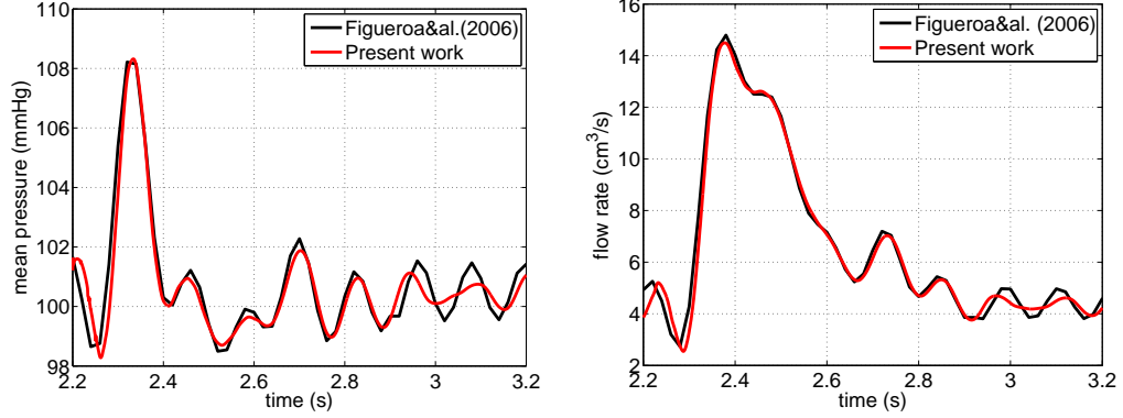
Figure 6: Mean quantities computed at S_1 and S_2 with constant pressure at outflow. Comparison between our results and those in [19]
