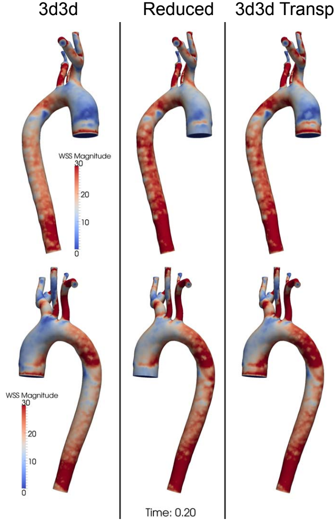
Figure 13: Pattern of the wall shear stress ( \text{dyn}/\text{cm}^2 ) near the systolic peak at time t=0.2 s. At the top: back view. At the bottom: front view
