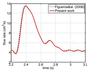
Figure 5: Flow rate at the section S_1 of the cylinder
