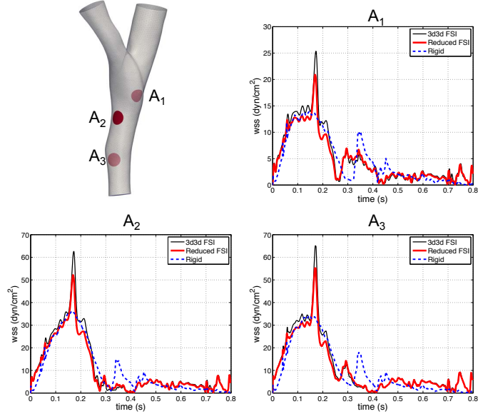
Figure 9: Mean wall shear stress ( \text{dyn/cm}^2 ) in time on three portions of the interface (coarse mesh). In red: reduced order FSI model. In black: 3D-3D FSI model. In blue: Navier-Stokes, rigid walls
