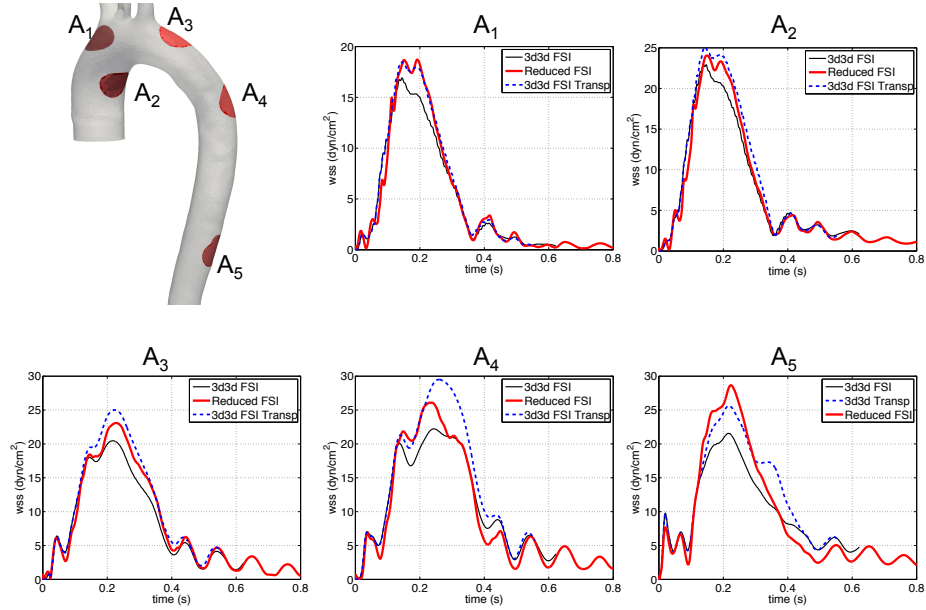
Figure 12: Mean wall shear stress ( \text{dyn/cm}^2 ) in time on five portions of the interface. In red: reduced order FSI model. In black: 3D-3D FSI model. In blue: 3D-3D FSI model with transpiration conditions
