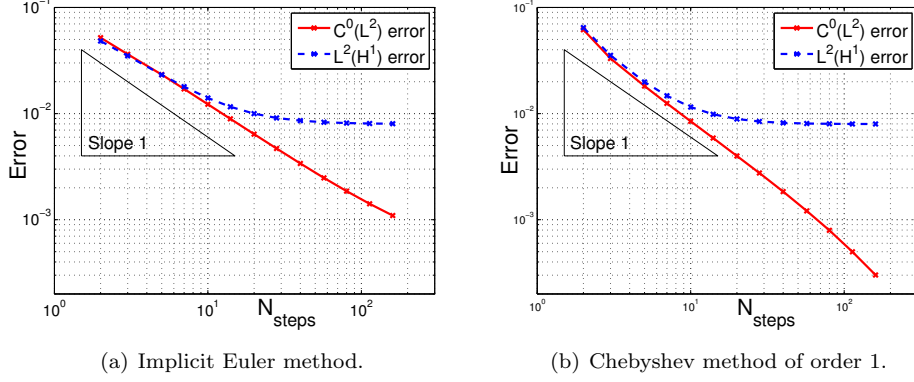
Fig. 1. Linear problem (6.2)-(6.5). e_{C^0(L^2),T} error (solid lines) and e_{L^2(H^1),T} error (dashed lines) versus the number N_{steps} of timesteps. Fine macro and micro meshes ( N_{macro} = N_{micro} = 128 ).
