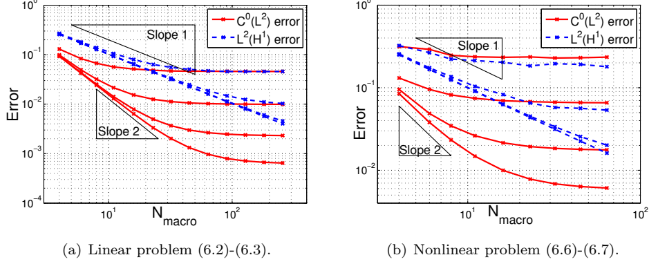
Fig. 2. e_{C^0(L^2),T} error (solid lines) and e_{L^2(H^1),T} error (dashed lines) versus N_{macro} . The lines correspond respectively to N_{micro} = 4, 8, 16, 32 .
