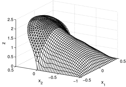
(c) FE-HMM with N_{micro} = 128 , \delta = 0.12 . 1100 DOF (for macro mesh).
