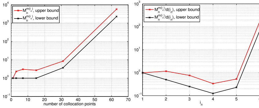
Fig. 5: The lower and upper bounds for \mathbb{M}_n^{m,SL(i_n)} for Gauss–Patterson points (left plot) and the corresponding ratios \mathbb{M}_n^{m,SL(i_n)}/d(i_n) are not bounded.
