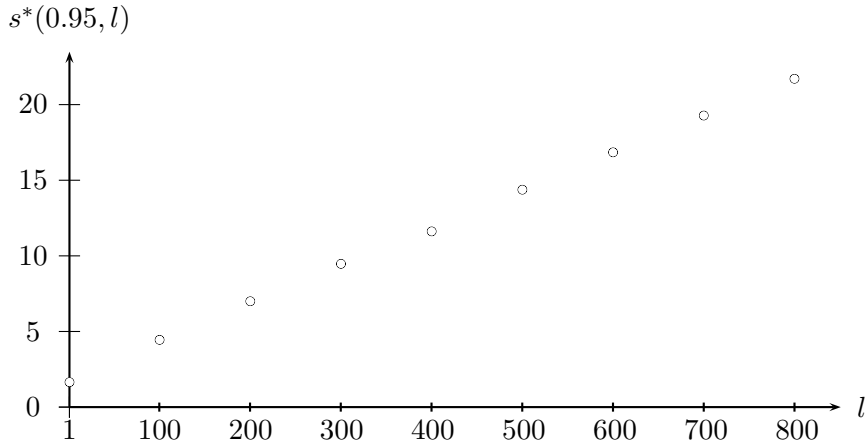
Figure 1: Values of s^*(0.95, l) for l = 1, 100, \dots, 800 .
