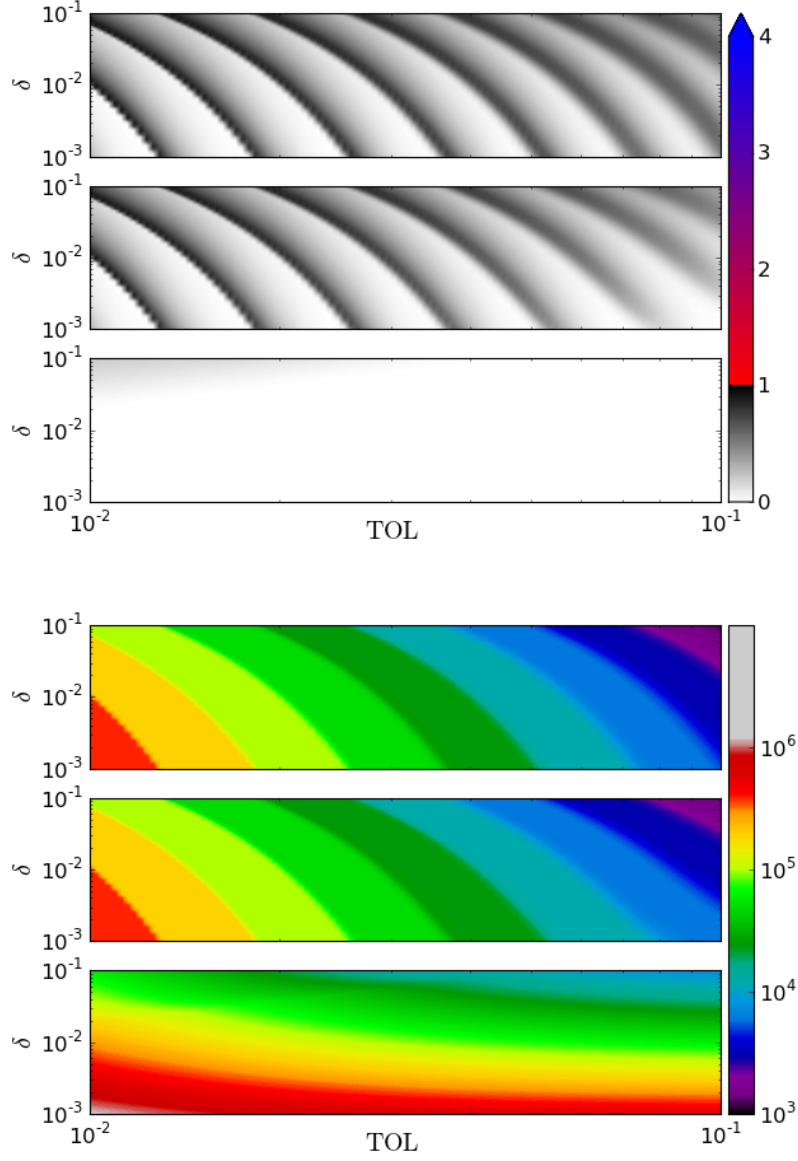
FIGURE 5. ( Exponential Distribution ) We sample an exponentially distributed r.v. with \mu = 1 . Top three plots: Plots of \bar{p}_N(\text{TOL}, \delta)/\delta , cf. (15), where samples of \bar{X}_M respectively are computed by Algorithm 1 in the top plot, Algorithm 2 in the middle plot, and Hickernell et al.'s algorithm in the bottom plot. We consider the algorithm unreliable at (\text{TOL}, \delta) points where \bar{p}_N/\delta > 1 . The bottom three plots are corresponding plots of the respective algorithms' complexity in terms of the average number of r.v. samples required to generate \bar{X}_M at the given (\text{TOL}, \delta) point.
