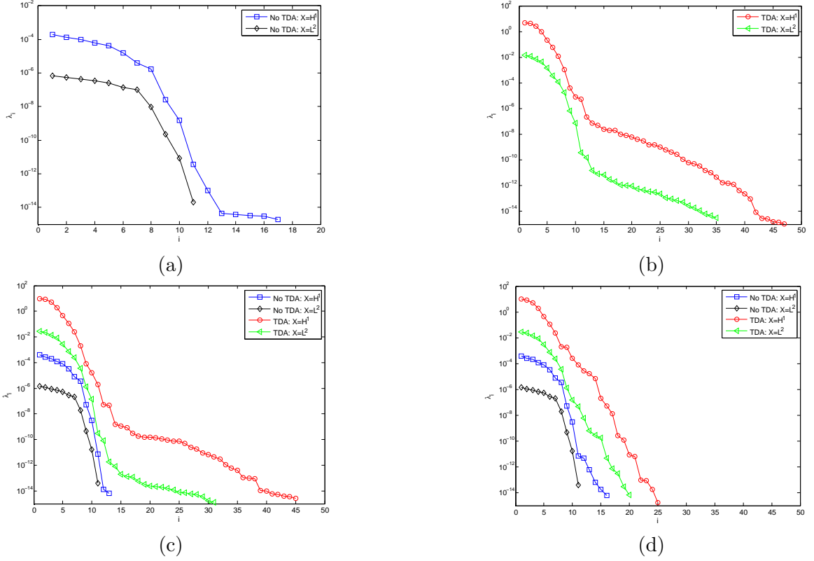
Figure 5: Decay of first few eigenvalues of correlation matrix obtained in X = L^2/H^1 and with/without TDQ for Example 5.2 ( h = 1/32 ): (a) p = 3 , k_m = 2 , N_x = 1225 (No TDA); (b) p = 3 , k_m = 2 , N_x = 1225 (TDA); (c) p = 4 , k_m = 3 , N_x = 1296 ; (d) p = 3 , k_m = 1 , N_x = 4356 .
