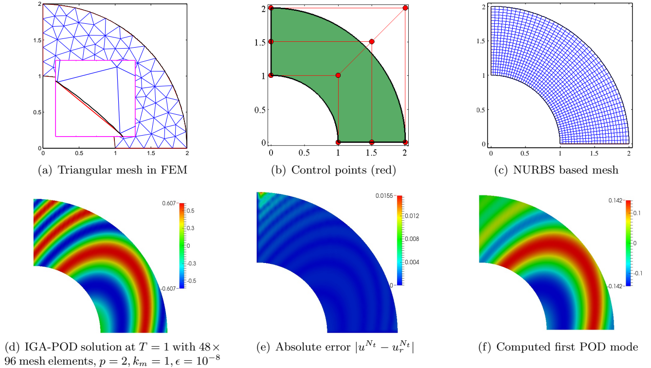
Figure 1: Triangulation, control points, NURBS based mesh, POD Galerkin solution, its error distribution and the first computed POD mode for Example 5.1.
