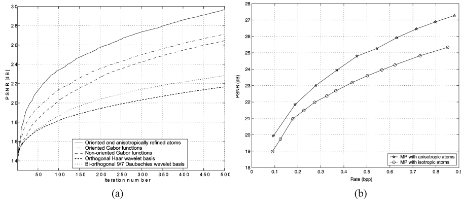
Fig. 4. Comparison of (a) the quality of MP approximation of Lena ( 128 \times 128 pixels), using five different dictionaries (anisotropic refinement and oriented functions, oriented Gabor wavelets, nonoriented Gabor wavelets or Weyl-Heisenberg dictionary, an orthogonal Haar wavelet basis and a biorthogonal Daubechies 9/7 basis, with five levels of decomposition) and (b) characteristic of anisotropic refinement in the dictionary. In (b), the basis functions used are the same for isotropic and anisotropic functions, with the same parameter discretization, showing the improvements of adding anisotropy to the dictionary.
