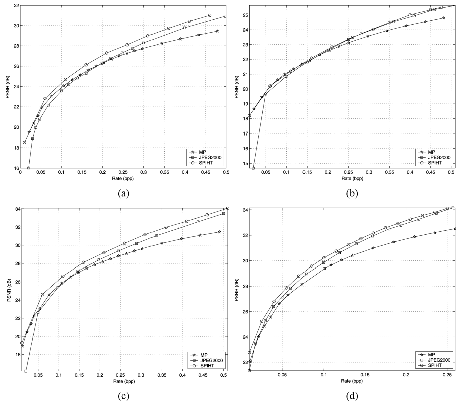
Fig. 5. Distortion-rate performance for JPEG2000, SPIHT and the proposed MP coder, for several test images. (a) Cameraman , 256 \times 256 . (b) Barbara , 256 \times 256 . (c) Lena , 256 \times 256 . (d) Lena , 512 \times 512 .
