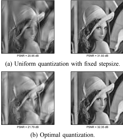
Fig. 2. Reconstructed Lena (128 x 128). Side reconstruction from the first description (left column) and central reconstruction (right column).
