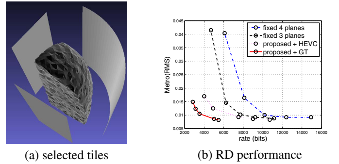
Fig. 4. Result for the second 3D mesh.
