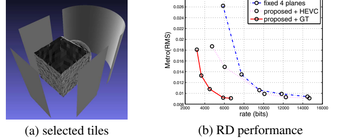
Fig. 3. Result for the first 3D mesh.
