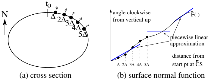
Fig. 2. Example of cross section and surface normal function.
