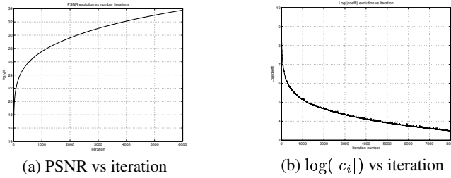
Fig. 2. PSNR and atom coefficient evolution vs iteration number
