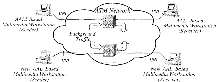
Figure 4: Simulation Setup
