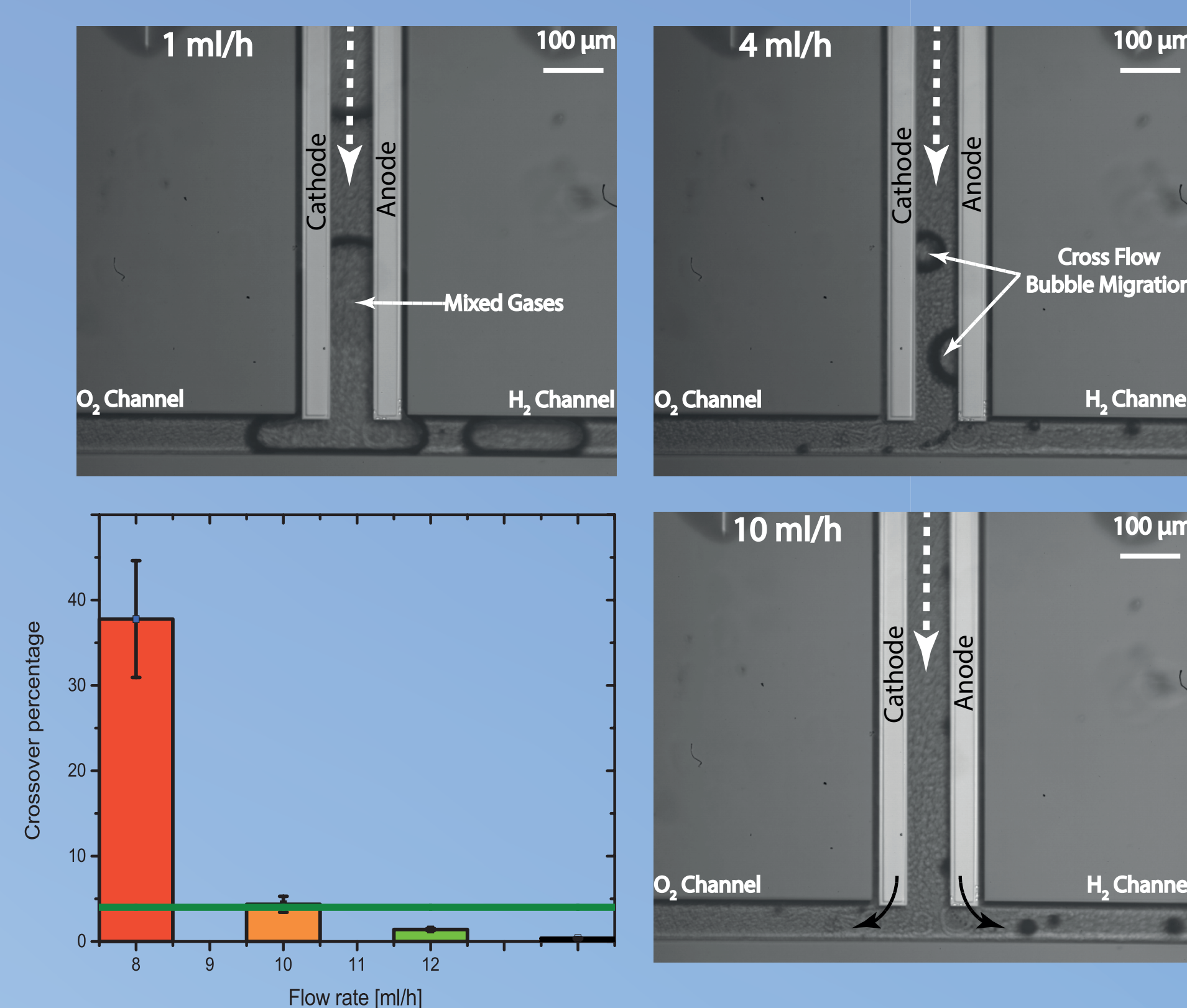
Effect of flow rate on gas crossover
