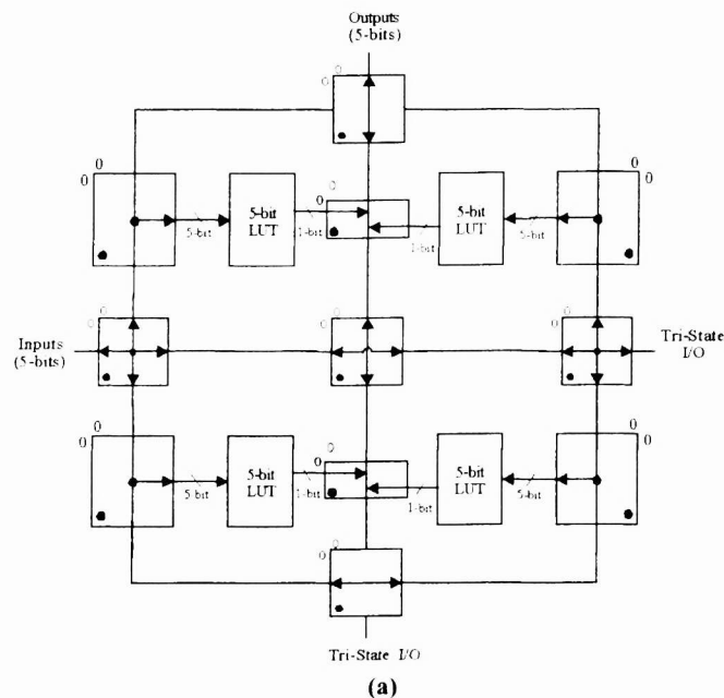
Figure 12. Logic block test: (a) The inputs of the 4 logic blocks are connected to the left crossbar matrix and the 4 outputs are routed out through the top matrix. (b) In the scopetrace, the chip is reset (Global_reset) before the logic block and interconnects are programmed (Parallel_Load). After configuration, the test input cycles through all the 5-bit states (during LUT Scan_Enable, but not shown). The LUT outputs logic 1 for only one state (5hex) and logic 0 for all the others (LUT Output)
