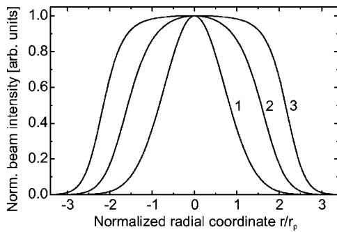
FIG. 3. Transverse beam profile (normalized intensities) for different values of the product \beta_p I_p^0 x . Lines 1, 2, and 3 are plotted for \beta_p I_p^0 x=0 (the input shape), 10, and 100.
