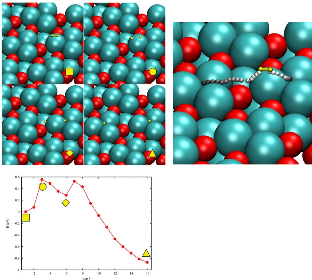
Figure S9: Hydrogen dissociation requires overcoming a barrier of 0.55 eV. The first minimum is due to one H atom in a metastable position.
