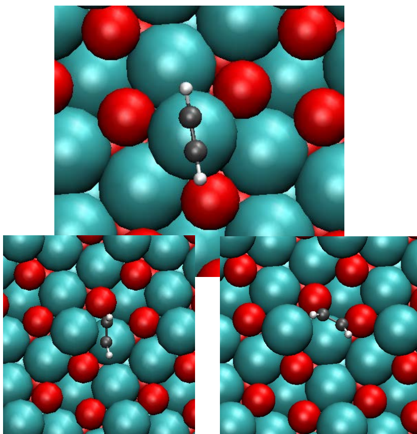
Figure S6: Three different adsorption configurations for C 2 H 2 on Pd 1 yielding adsorption energies of 0.61 eV, 0.43 eV and 0.60 eV for the situations shown in the top, bottom left, and bottom right panel, respectively.
