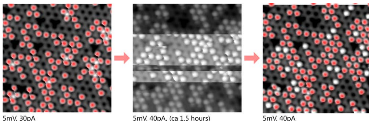
Figure S3: Tip induced relaxation of C_2H_2 adsorbed in the interstitial adsorption site on Pd_1 . A slight increase in tunneling current (30 pA \rightarrow 40 pA) first leads to unstable imaging conditions and tip changes (center). After scanning the same area for about 1.5 hours, conditions have stabilized and almost all interstitial adsorbates have disappeared. Instead the number of on-top adsorbed C_2H_2 has increased. Protrusions that were present initially are marked in red.
