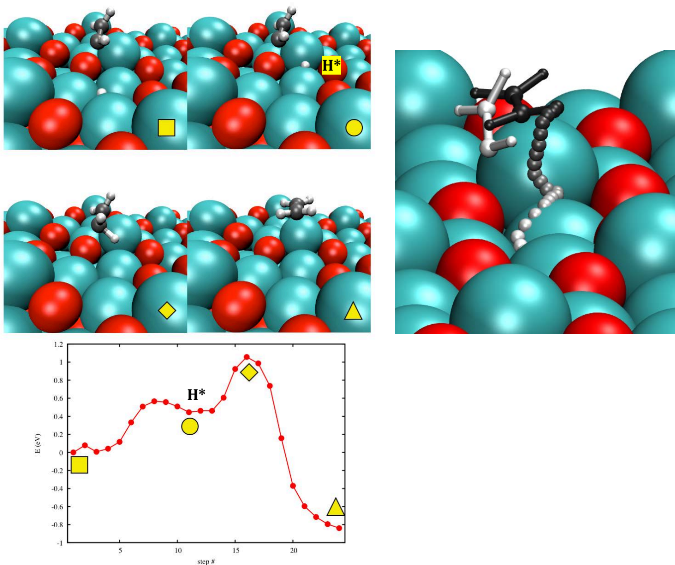
Figure S15: In the case of Pd_1 , we split the NEB in two different calculations to test the diffusion of atomic hydrogen. To reach the metastable position (●), an initial barrier of 0.6 eV has to be overcome. The following the attack of the vinyl fragment yields a further barrier of 0.6 eV leading to the more stable ethylene state on-top of the outermost Pd atom (▲).
