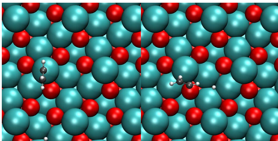
Figure S8: The configuration shown in the right panel is more stable by 0.66 eV compared to the on-top Pd position shown in the left panel. As for C_2H_2 , adsorption (see Figure S6), an adsorption site involving 2 nd layer Ga atoms is identified for this surface.
