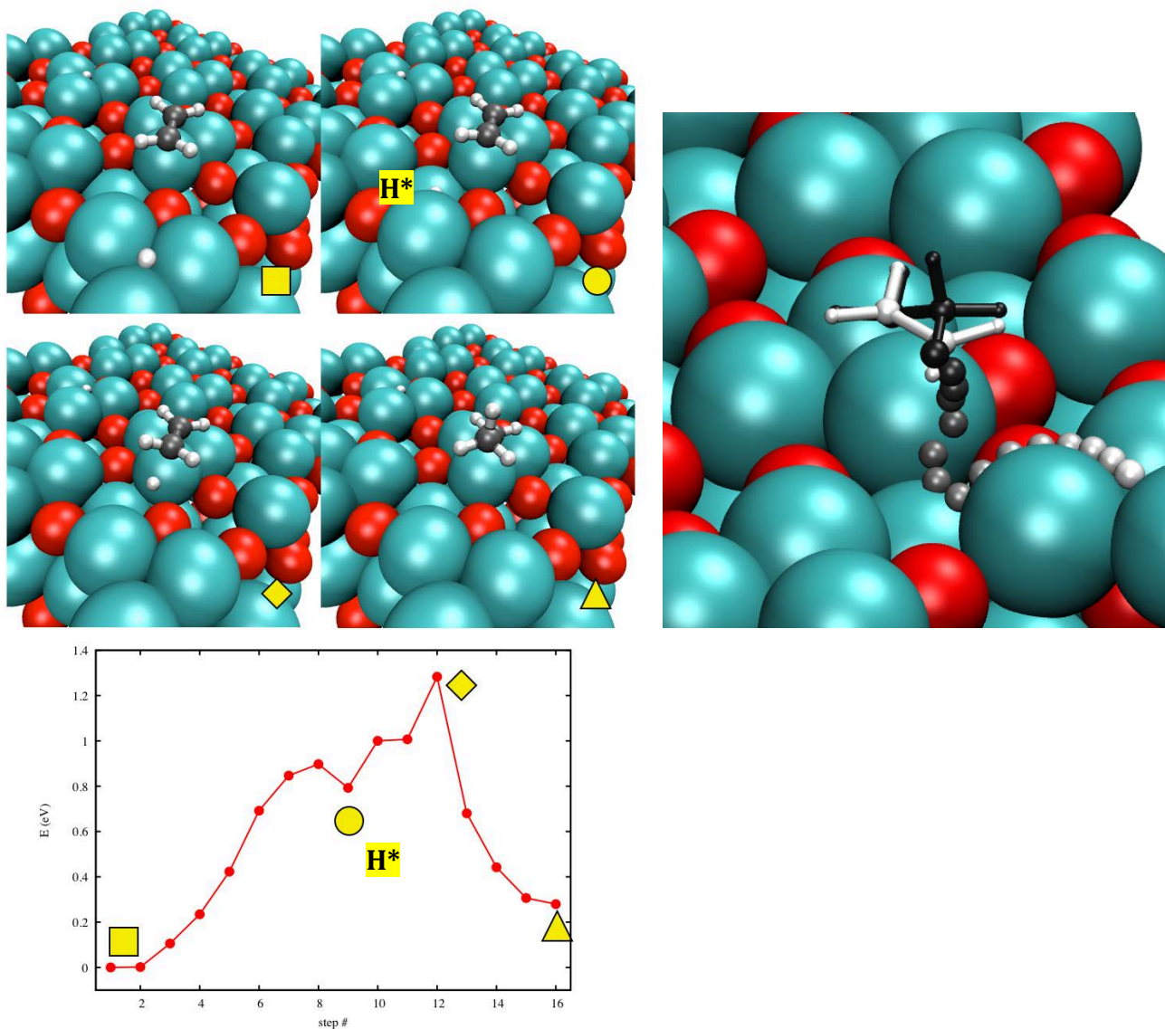
Figure S16: Also here we consider the two processes in the NEB, starting with an approach of the hydrogen atom from the absolute minimum (■) to a metastable position of hydrogen ( H^* , 0.8 eV) and the subsequent hydrogenation step to C_2H_5 with a total barrier height of 1.3 eV.
