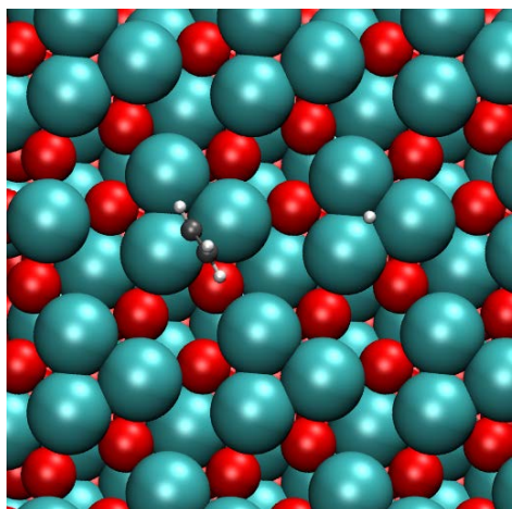
Figure S7: The favored adsorption site after the first hydrogenation step is a bridge site between two Pd atoms of the trimer, yielding only a small energy gain of 0.076 eV with respect to C_2H_2 . The C-C axis of the C_2H_3 molecule is tilted with respect to the surface plane.
