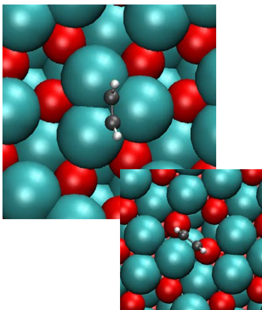
Figure S5: Top: Favored adsorption configuration for C 2 H 2 on Pd 3 , which is very similar to the one found on Pd(111). The inset shows the adsorption on the Ga atoms of the 2 nd layer, similar to that found for Pd 1 (see Figure S6). However, on Pd 3 this configuration yields an adsorption energy of only 0.3 eV, and is thus unfavorable.
