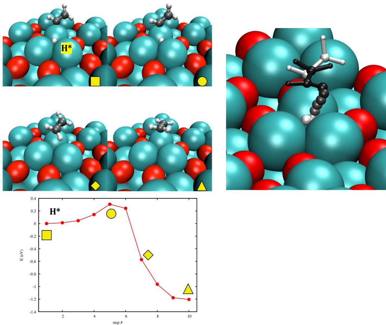
Figure S14: To achieve hydrogenation, the hydrogen has to diffuse in an endothermic step ( H^* , 0.5 eV) to the trimer hosting the vinyl (■). The co-adsorption on the same trimers leads to a shift of the vinyl from the preferred bridge site (Figure S7) to an on-top site position on Pd. The NEB presented above starts from this situation, yielding a reaction barrier of 0.3 eV for the hydrogenation step(●).
