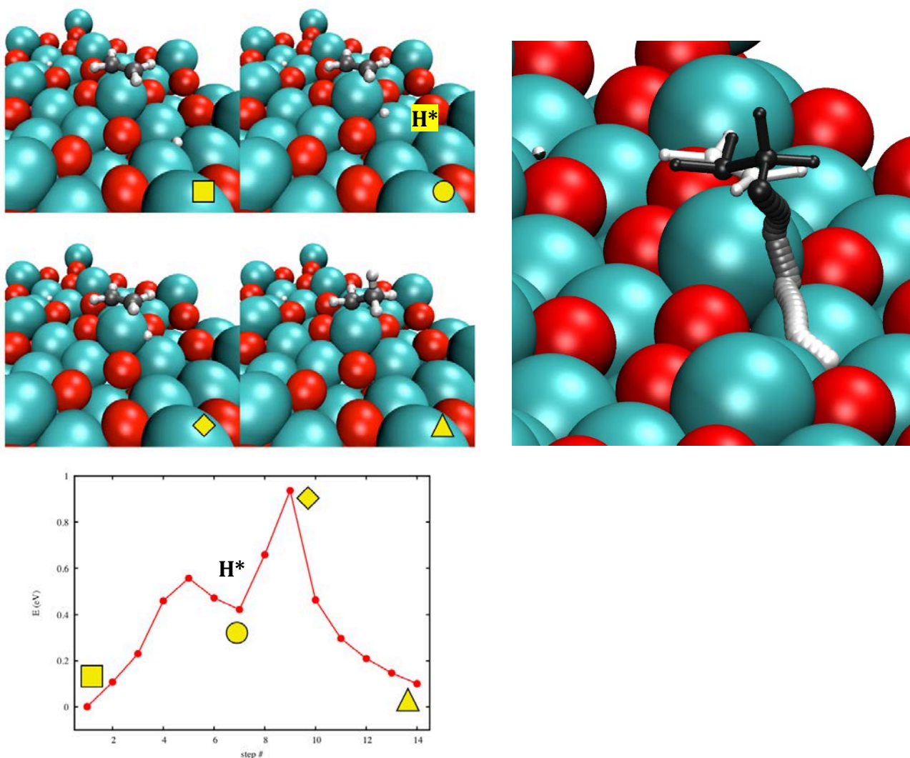
Figure S17: Also for Pd_1 , we include the hydrogen approach in the NEB simulation. The total barrier amounts to 0.9 eV, including the diffusion of H to the metastable position (●) at 0.4 eV, and the subsequent hydrogenation step with a barrier of 0.5 eV. As explained in the manuscript, desorption of ethylene (which has a lower adsorption energy of 0.73 eV) is likely to occur before the barrier for transformation to C_2H_5 is overcome.
