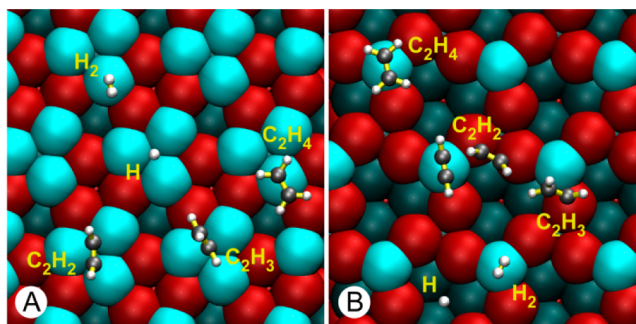
Figure 2. Summary of the DFT optimized, minimum energy adsorption configurations for various molecules on the \text{Pd}_3 (A) and the \text{Pd}_1 (B) surfaces, respectively. (Pd: cyan, Pd(subsurface): dark cyan, Ga: red, C: black). Most adsorption sites are located on the topmost Pd atoms.
