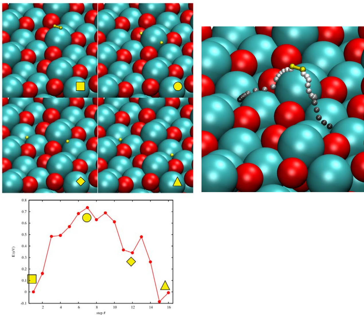
Figure S10: The barrier for hydrogen dissociation on Pd_1 is computed to 0.72 eV, with only a small gain in total energy.
