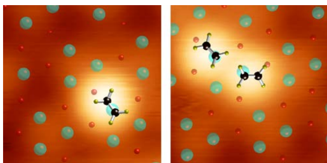
Figure S4: Steric repulsion of neighboring C_2H_4 molecules adsorbed on the same Pd trimer on PdGa:A(-1-1-1)Pd_3 . The adsorption energy per molecule accounts to 0.69 eV and 0.50 eV for the left and right case, respectively.
