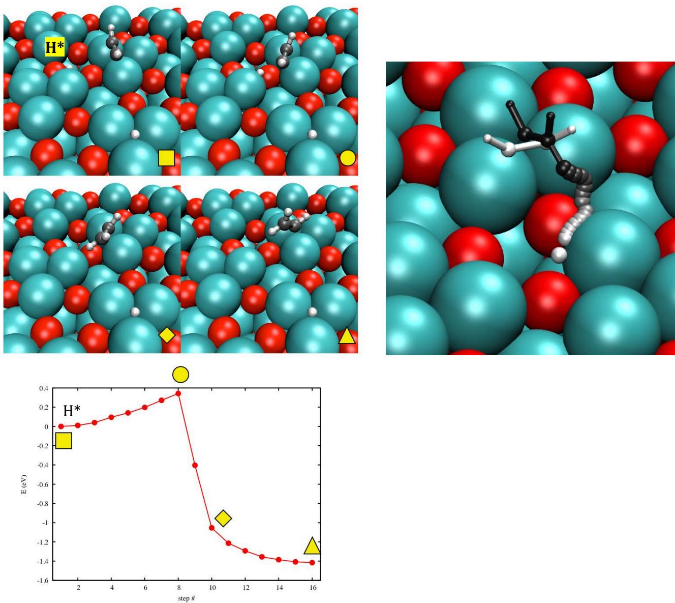
Figure S11: The first hydrogenation step on Pd_3 requires a precedent endothermic (0.7 eV) approach of the atomic hydrogen towards the hydrocarbon (not shown in the graph) into a metastable position H^* . The hydrogenation barrier from the metastable hydrogen position is very low with 0.34 eV.
