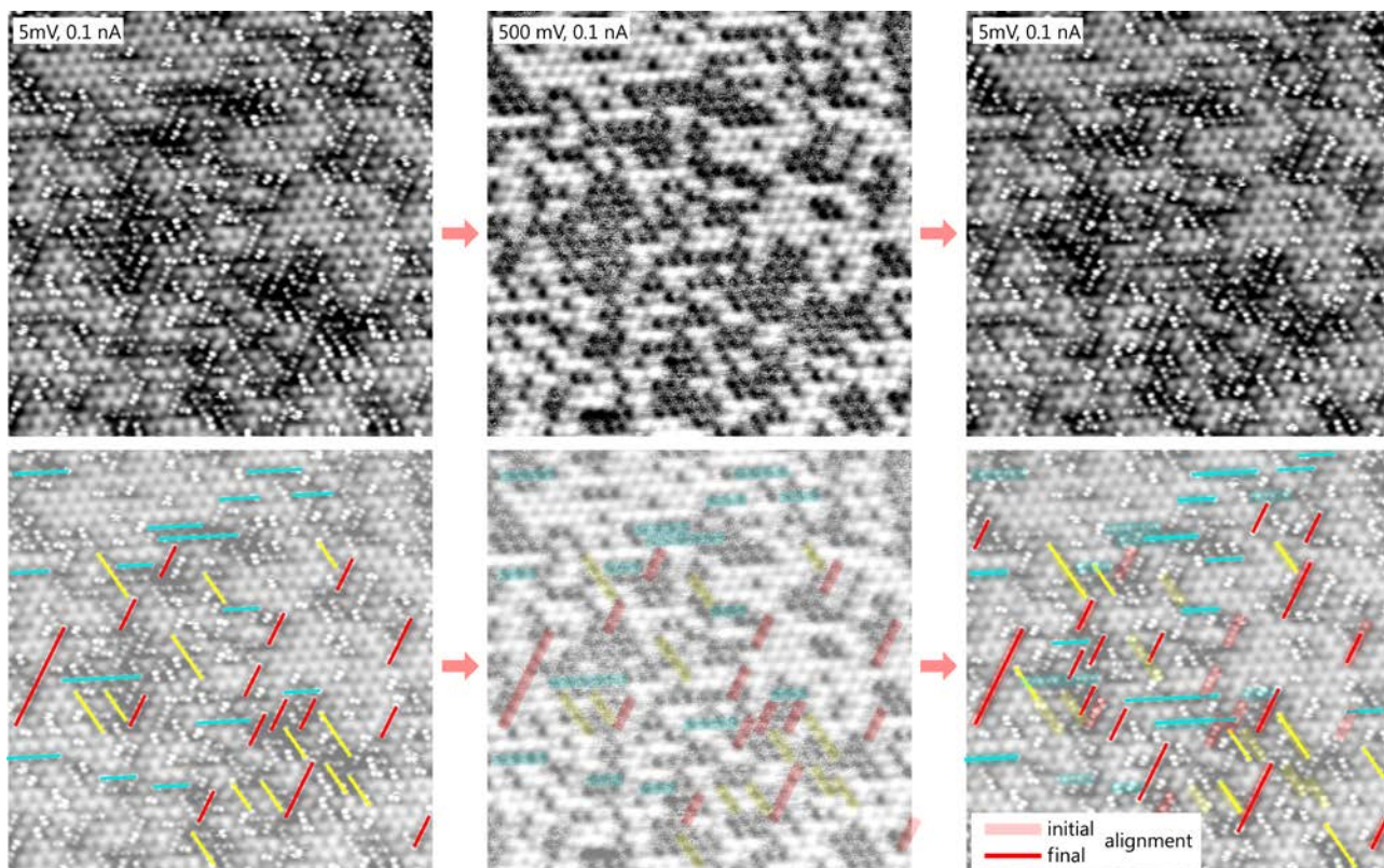
Figure S2: Top: Three subsequent STM images (20 x 20 nm) of C 2 H 2 molecules on PdGa:A:(-1-1-1)Pd 3 at 5 K. Bottom: alignments of three or more adsorbates are marked with colored lines, color coded for the three symmetry-equivalent directions. Middle: Increasing the tunnel voltage from 5 mV to 500 mV leads to a re-arrangement of the collective orientations.
