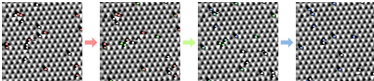
Figure S1: Tip induced hopping of H 2 molecules on the Pd 3 surfaces at 5K. Images were taken in upwards scan with a period of 1 minute. As a guide to the eye, those molecules that maintain their position in two subsequent images are color coded. (10 x 10 nm, tunnel parameters: - 5 mV, 1nA)
