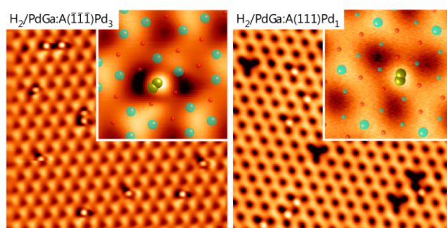
Figure 1. STM images ( 10 \times 10 nm) of \text{H}_2 adsorbed at T = 5 K on \text{PdGa:A}(-1-1-1)\text{Pd}_3 (left) and on \text{PdGa:A}(111)\text{Pd}_1 (right). The hexagonal periodicity of the topmost atomic layers of the two three-fold surfaces is visible. Insets show a magnified section ( 1.5 \times 1.5 nm) of a single molecule. The superimposed atomic ball models show the lowest energy adsorption configurations as determined by DFT (Pd: cyan, Ga: red, H: yellow). For clarity, the atoms of the terminating layers and H are drawn with enlarged radii. In the right panel, the surface vacancy defects typical for the \text{Pd}_1 termination 11 appear as dark, three-fold features. (Tunneling parameters: left: -5 mV, 1 nA; right: 5 mV, 20 pA).
