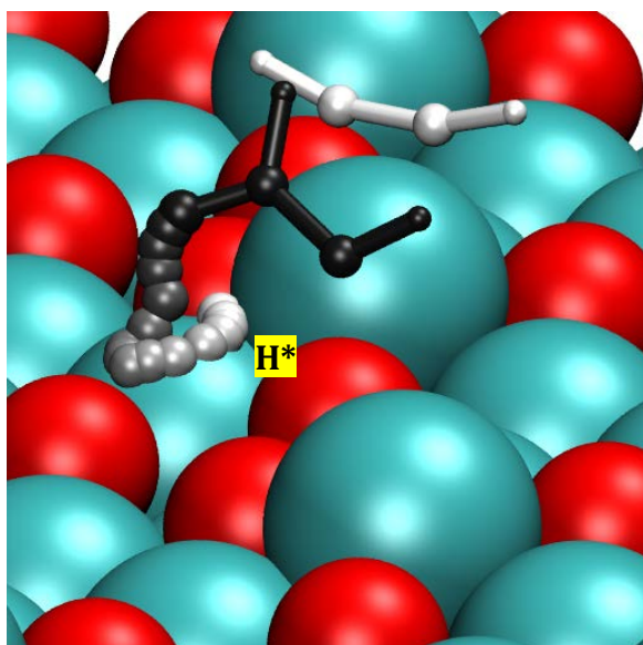
Figure S13: The second NEB path is connecting the on-top \pi configuration for \text{C}_2\text{H}_2 (Figure S6, top panel) with the bridge site energetic minimum of \text{C}_2\text{H}_3 (Figure S8, right panel). (This reaction barrier is not shown in Figure 7 of the main text.) The hydrogenation barrier amounts to 0.62 eV. The precedent hydrogen approach step (not shown) would cost additional 0.6 eV, which makes this reaction path less likely than the one starting from \text{C}_2\text{H}_2 in a \pi/\text{di-}\sigma Ga bridge state, shown in Figure S12.
