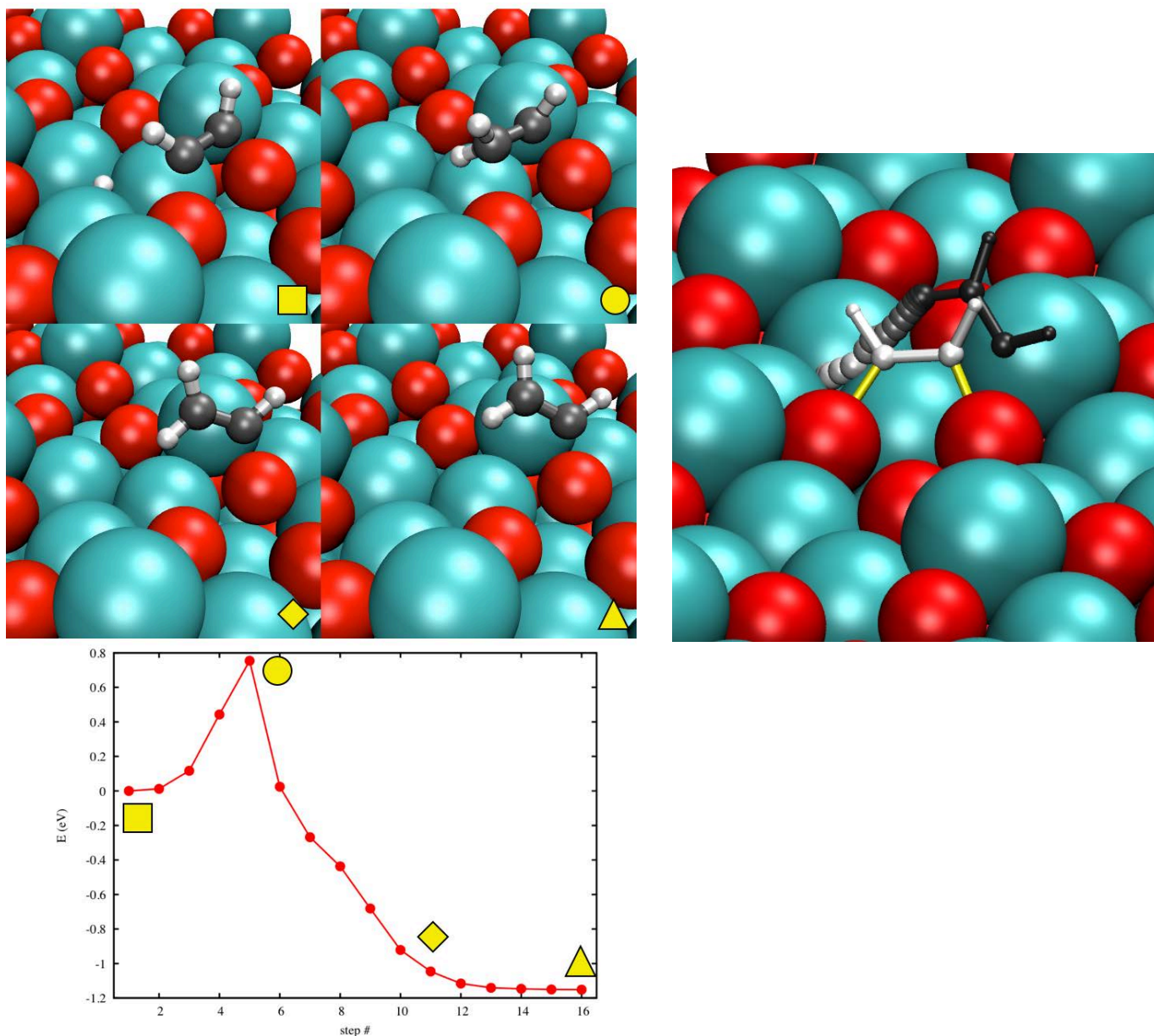
Figure S12: The first NEB simulated reaction connects the alternative \pi /di- \sigma Ga configuration for acetylene (Figure S6, bottom right panel) to the favorable adsorption geometry for C_2H_3 (Figure S8, right panel). As the hydrogen is supplied from the hollow site of the 3 rd layer Pd trimer, no additional barrier is present for the hydrogen approach.
