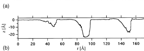
FIG. 7. (a) STM topograph of Al(111) recorded after exposure of 20 L O_2 and 5 min. annealing at 515 K. 266 \text{ \AA} \times 212 \text{ \AA} ; -0.37 \text{ V} , 20 \text{ nA} . (b) Profile along the line indicated in (a).
