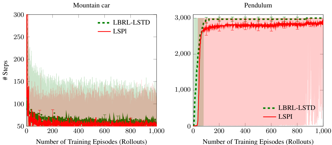
Figure 2: Online performance comparison between LBRL-LSTD and LSPI. The error bars show 95% confidence intervals, while the shaded regions show 90% percentiles over 100 runs.
