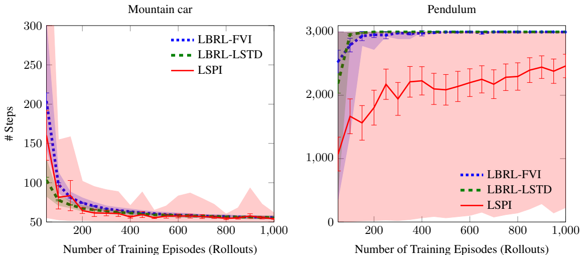
Figure 1: Offline performance comparison between LBRL-FVI, LBRL-LSTD and LSPI. The error bars show 95% confidence intervals, while the shaded regions show 90% percentiles over 100 runs.
