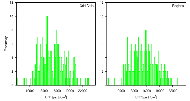
Figure 3: Distribution of the annual average UFP concentrations of (left) the top 200 grid cells with most measurements; and (right) the top 200 regions with most measurements
