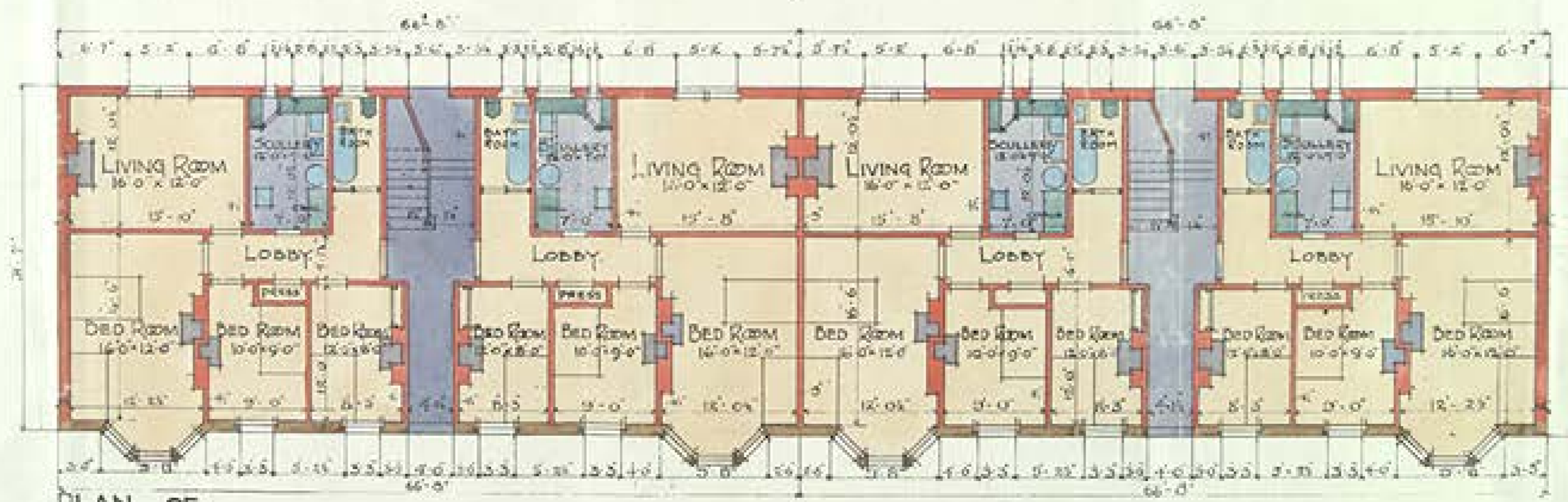
PLAN OF GROUND FLOORS.
