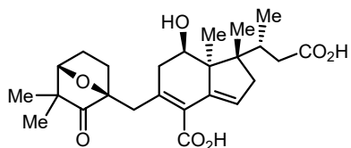
glycinoclepin A
