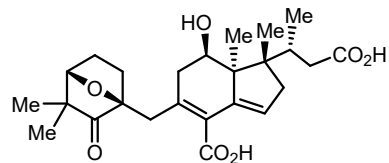
glycinoclepin A
