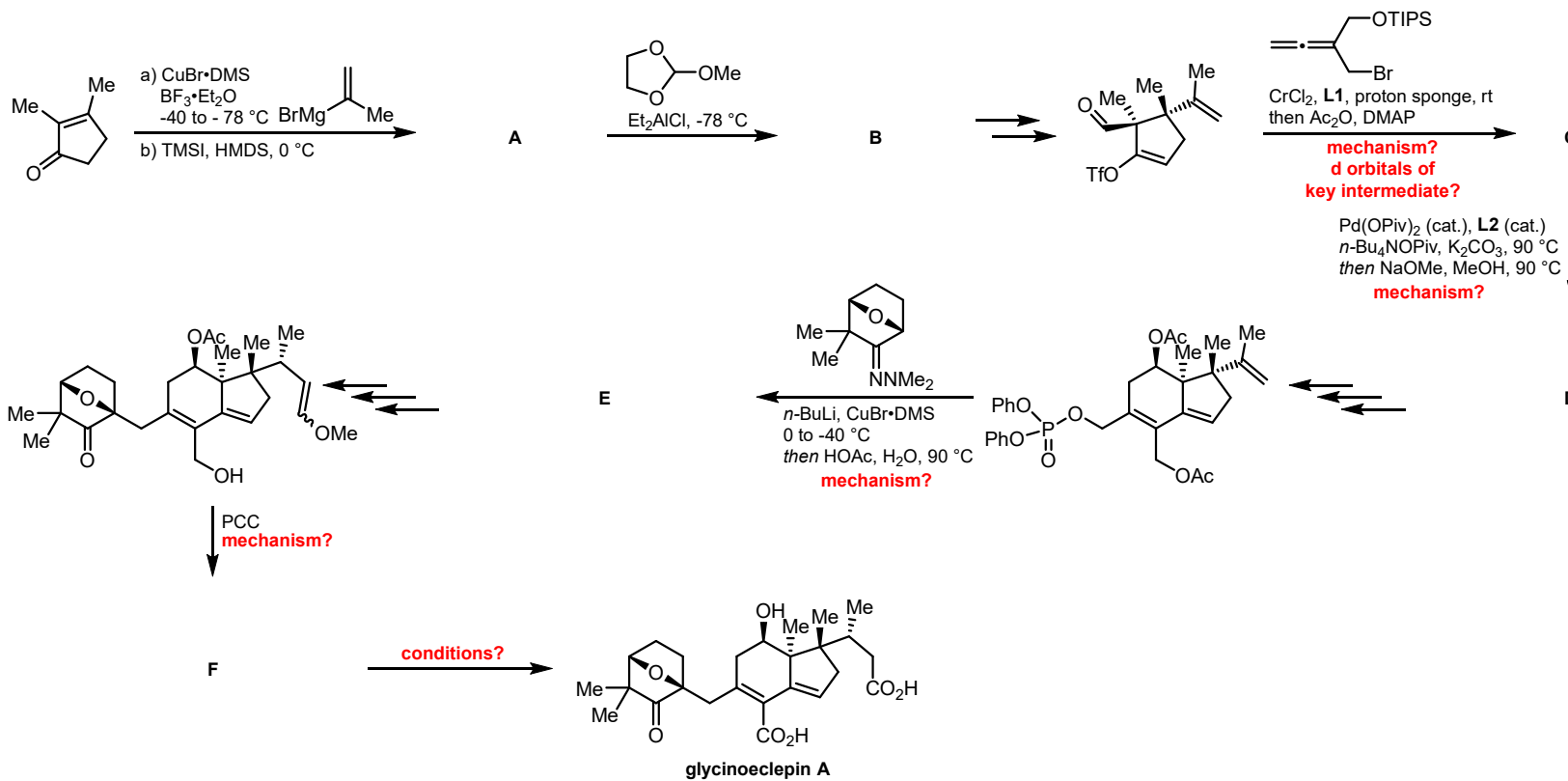
glycinoclepin A
