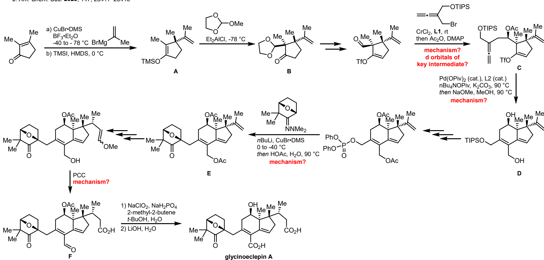
glycinoclepin A
