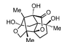
(–)-illisisimonin A (1)
