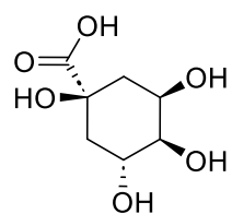
D-(-)-quinic acid
