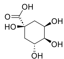
D-(-)-quinic acid
