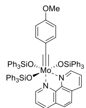
Fürstner's catalyst
