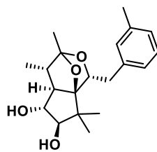
Mollebenzyolanol A, Ito, Org. Lett. 2020, 22, 7609–7612
