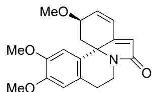
(±)-erysotramidine
