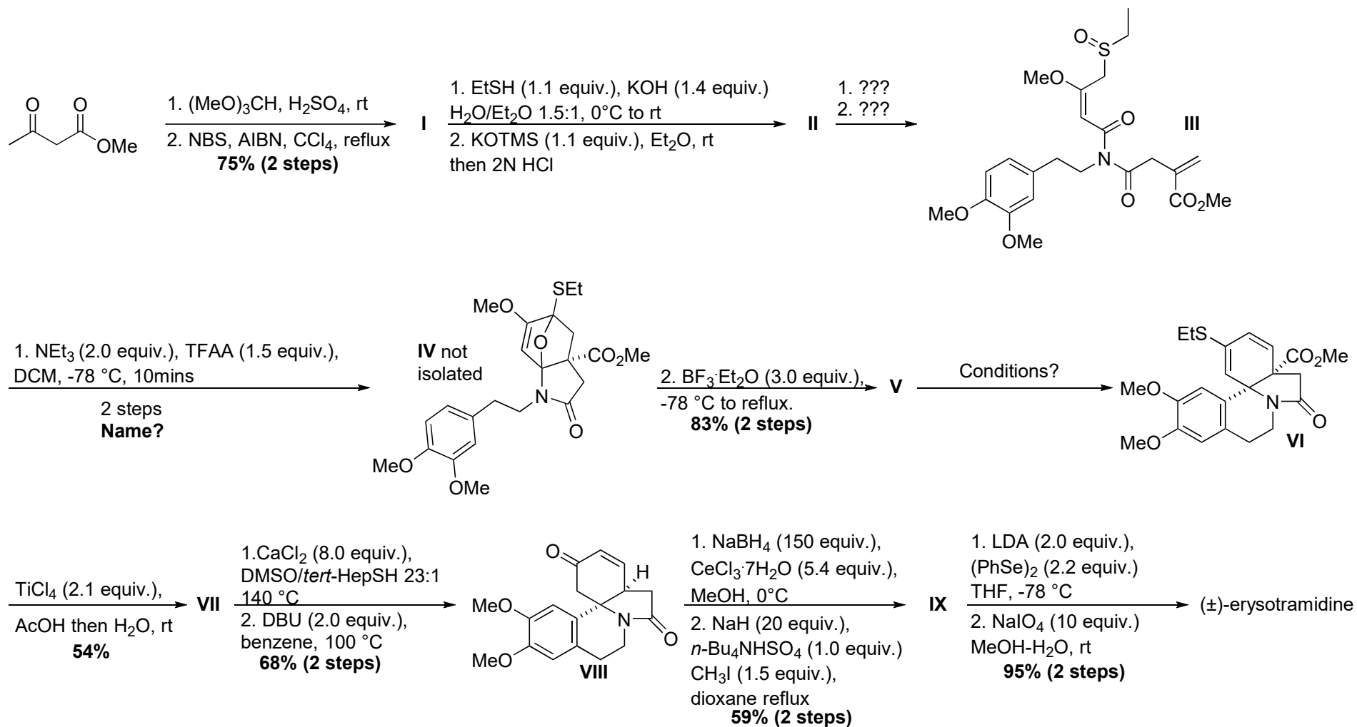
(±)-erysotramidine
