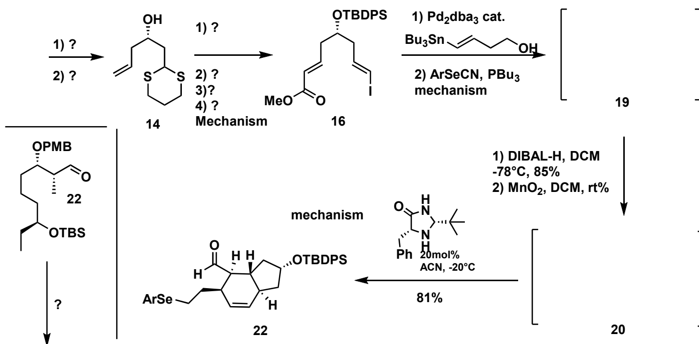
(-) Spinosin A JACS, 2016, 138, 10838-1041 23 steps total
