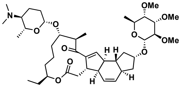
(-) Spinosin A JACS, 2016, 138, 10838-1041 23 steps total
