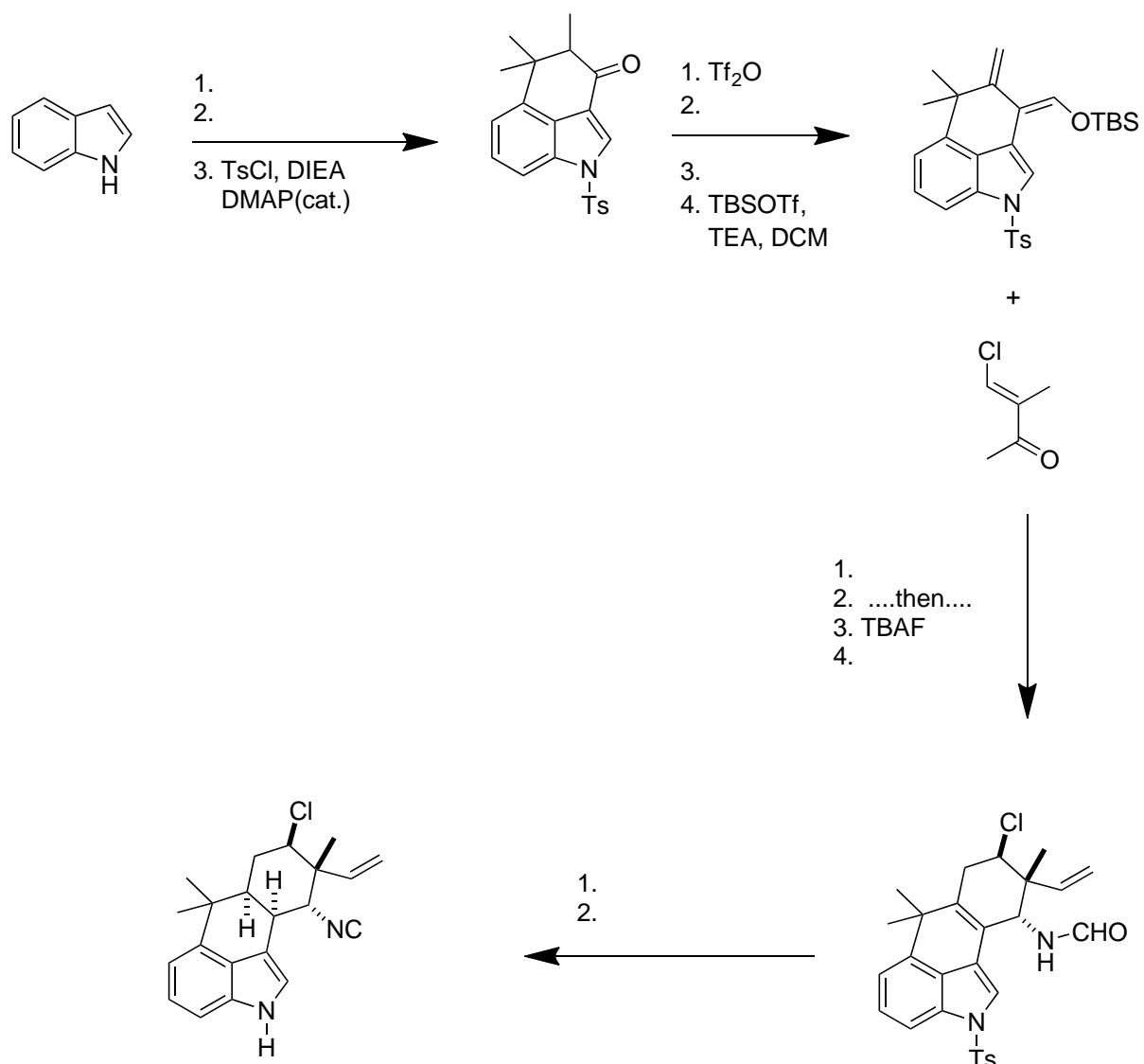
Hapalindole K
