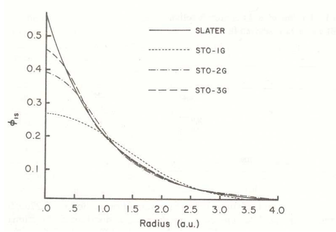
Figure 3.2: Comparison of the quality of the least-squares fits of a 1s Slater function ( \zeta = 1.0 ) obtained at the STO-1G, STO-2G, and STO-3G levels.
