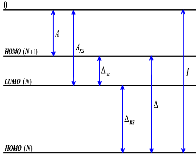
Figure 8.1: Schematic description of some important Kohn-Sham eigenvalues relative to the vacuum level, denoted by 0, and their relation to observables. See main text for explanations.
