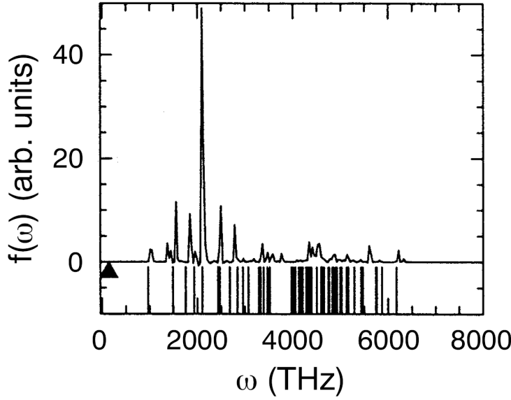
Figure 9.1: Vibrational density of states Eq. 9.14 (continuous spectrum in upper part) and harmonic approximation thereof (stick spectrum in lower part) of the electronic degrees of freedom compared to the highest frequency phonon mode \omega_n^{\max} (triangle) for a model system.
