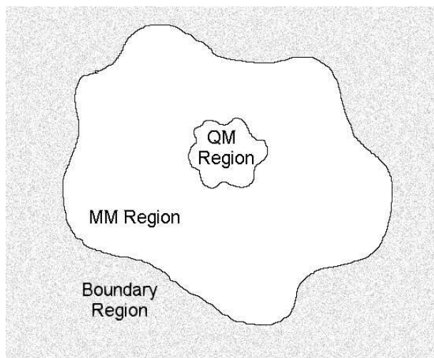
Figure 10.1: Cartoon representing a simple QM/MM setup. The central QM region can become the active site of an enzyme, the MM region the protein matrix, and the boundary region the solvent.
