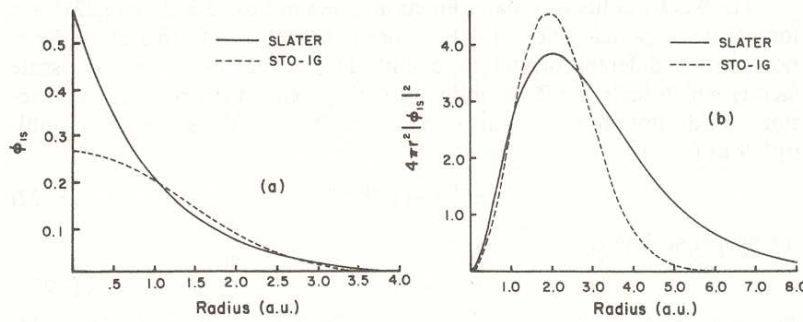
Figure 3.1: Comparison of Slater function with Gaussian function: a) least squares fit of a 1s Slater function ( \zeta = 1.0 ) by a single STO-1G 1s Gaussian function; b) comparison of the corresponding radial distribution functions ( 4\pi r^2 |\phi_{1s}(r)|^2 ).
