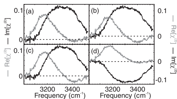
FIG. 5. Simulation of distortions induced by experimental or computational effects: (a) undistorted PS-SFG spectrum from Fig. 4(b), (b) distortion induced by a phase shift of 10^\circ , (c) distortion induced by a phase drift of \exp[i\omega t] of 40 fs, and (d) complex conjugation of the spectrum.
