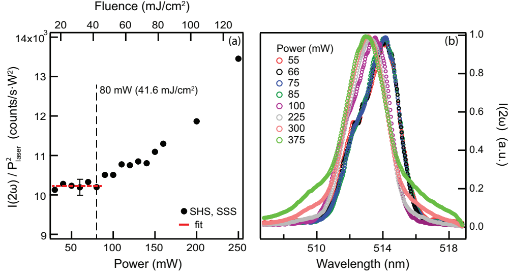
Figure 2.4: Elastic SHS of water. (a) SH intensity measured at 90° and divided by the square of the incident average power as a function of incident average power (bottom axis) and fluence (top axis). The red lines highlights the range in which there is a quadratic dependence of the SH intensity on the incident average power. (b) Normalized spectra of water at different incident powers at 90°. Courtesy of Y. Chen and C. Macias.
