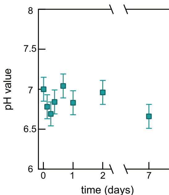
Figure 2.14: The pH stability of aqueous solutions over time. pH was measured in 10\ \mu\text{M} NaCl solutions that were stored in closed screw-cap vials in contact with an N_2 atmosphere. Courtesy of H. Okur.
