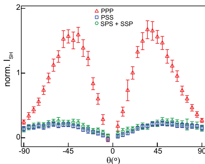
Figure 2.9: Scattering patterns of polystyrene beads Scattering patterns of 200 nm polystyrene beads in 3 polarization combinations PPP, PSS, SPS and SSP. The same magnitudes indicate that the assumption of the degeneracy of the susceptibility elements is correct. Error Bars represent the standard deviation of 20 measurements.
