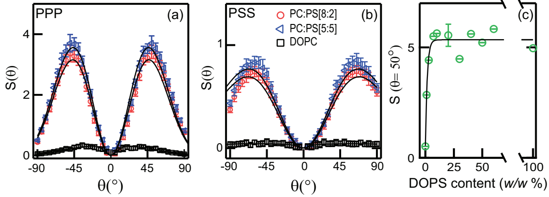
Figure 6.1: (a) SH scattering patterns in the PPP polarization combination. (b) SH scattering patterns in the PSS polarization combination. The lines represent fits made to the nonlinear Rayleigh-Gans-Debye theory from which the surface potential values were extracted using the parameters of Table 6.1 (c) Maximum SH intensity as a function of DOPS weight percentage in the liposomes (in the PPP polarization combination). The solid line is a guide for the eye.
