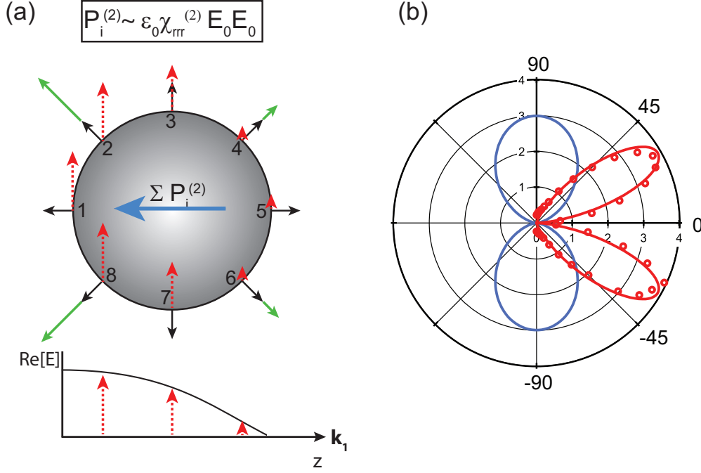
Figure 1.7: Second harmonic scattering from a sphere. (a) Schematic of the effect of relative size on nonlinear light scattering. A single beam impinges (z-direction) on a particle that has a surface susceptibility \chi_{rrr}^{(2)} \neq 0 indicated by black radial directed arrows. While propagating through the particle the phase of the incoming beam changes at different positions of the particle leading to different magnitudes of induced local polarizations (green arrows). The effective particle polarization is the sum of all induced polarization components resulting in a net longitudinal dipole along beam propagation. (b) Blue: simulated radiation pattern of the longitudinal dipole as drawn in (a). Red: Typical SHS pattern as observed in the far-field of 500 nm polystyrene beads solution in water with fit considering geometrical interference effects.
