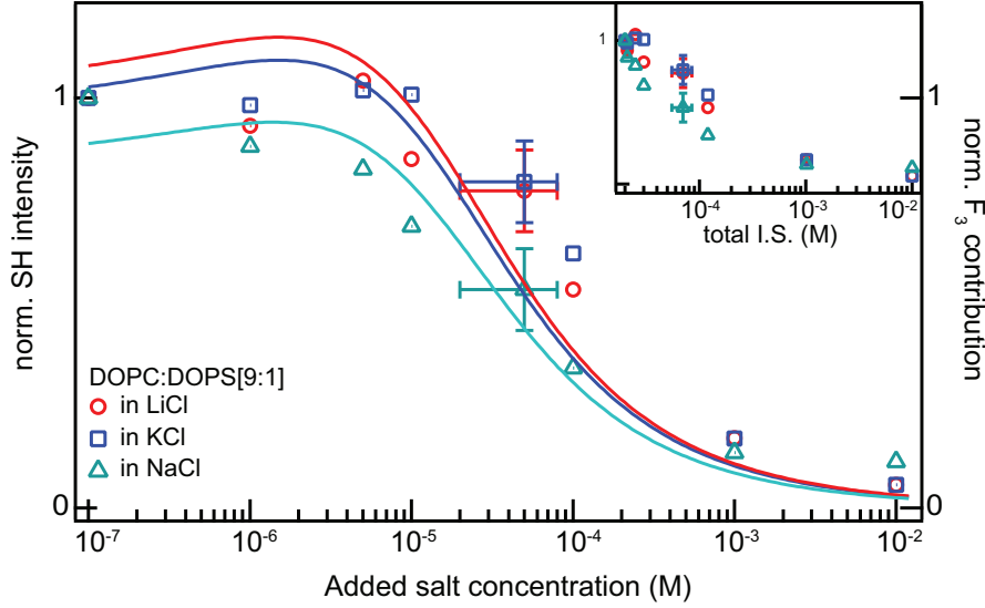
Figure 4.3: SH intensity trend at a fixed scattering angle \theta = 50^\circ as a function of added salt concentration for three monovalent salts: LiCl, KCl and NaCl. The computed trend for the F_3 -contribution is laid on top. Inset: The same data plotted for overall ionic strength of the sample and not just added salt concentration.
