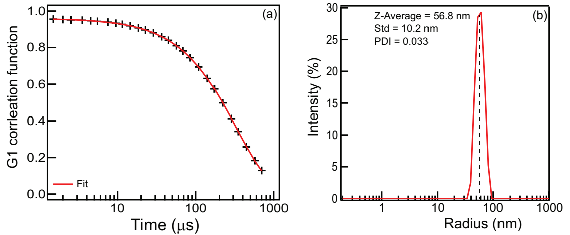
Figure 2.11: Size extraction from DLS measurements. (a) The size is determined by fitting the beginning of the correlation data with a cumulant fit considering a monodisperse solution, here for DOPS liposomes in water extruded through 100 nm pores. Deviations from this fit become apparent in the width of the displayed distribution and are expressed in the PDI. (b) The extracted typical size distribution showing a very low PDI calculated from the fit in panel (a).
