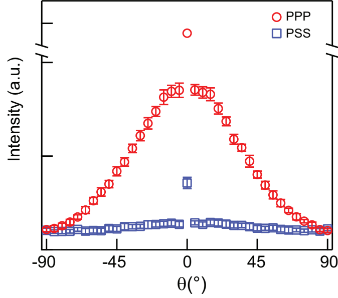
Figure 2.6: Scattering patterns of water in the PPP and PSS polarization combinations. 0^\circ corresponds to the forward propagation direction of the fundamental beam. The patterns were recorded in steps of 5^\circ with an angle of acceptance of 3.4^\circ . Error bars represent the standard deviation from 20 measurements per angle.
