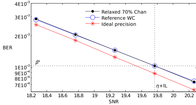
Fig. 8. Identical performance. BER simulation over 400 channels different from the training set. The simulation shows no meaningful performance difference between our adaptive approach and the worst-case design.
