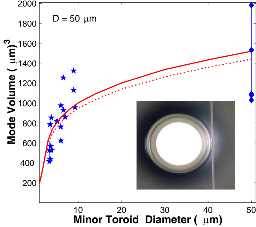
Figure 9.7: Main figure: Experimental and theoretical mode volume (in cubic-microns) of toroid microcavities as a function of the toroid minor diameter ( d ) for fixed principal diameter D ( D=50 microns). The case d=D (unity aspect ratio) corresponds to a microsphere, and the data shown for this case is taken from ref [89] for comparison. The solid and dotted lines refer to the mode volume of a fundamental toroidal WGM (TM and TE case respectively) obtained by numerical modeling. Inset: An optical micrograph of a ca. 80-micron-diameter toroid microcavity coupled to a tapered optical fiber.
