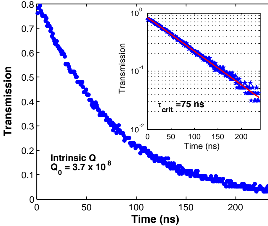
Figure 7.8: Cavity ringdown measurement of a toroid microcavity with a free spectral range \Delta\lambda_{FSR} = 7.3 \text{ nm} . The main figure shows the cavity decay signal at the critical coupling point, exhibiting a critical decay time of 75 ns (which corresponds to 0.98 \times 10^8 ). When correcting for waveguide loading ( \Gamma \approx 3 ) the intrinsic Q-factor yields 3.7 \times 10^8 . The corresponding finesse of the cavity is F = \Delta\lambda_{FSR}/\Delta\lambda = 1.74 \times 10^6 .
