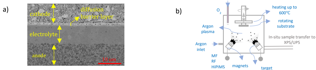
Figure 1. a) Cross-section view of a SOFC, showing diffusion barrier layer, b) Schematic of reactive magnetron co-sputtering
