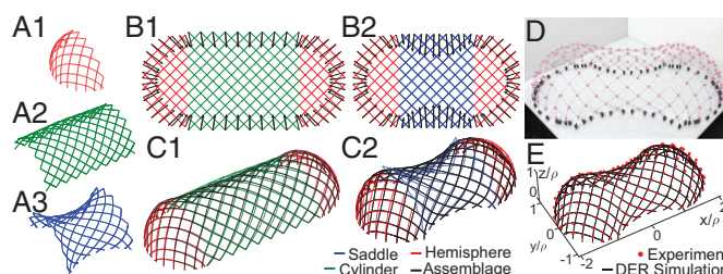
Fig. 5. Elastic gridshells from building blocks. (A) Pruned elastic gridshell building blocks: (A1) hemisphere, (A2) cylinder, and (A3) saddle. (B and C) Comparison of concatenated elastic gridshell assemblage (black solid lines) and its building blocks (colored solid lines) for (B1 and C1) stadium (A1-A2-A1) and (B2 and C2) peanut (A1-A3-A1). (D) Photograph of a peanut-shaped elastic gridshell. (E) Positions of the joints (red solid circles; 3D scanning), along with the corresponding DER simulation (black solid lines).
